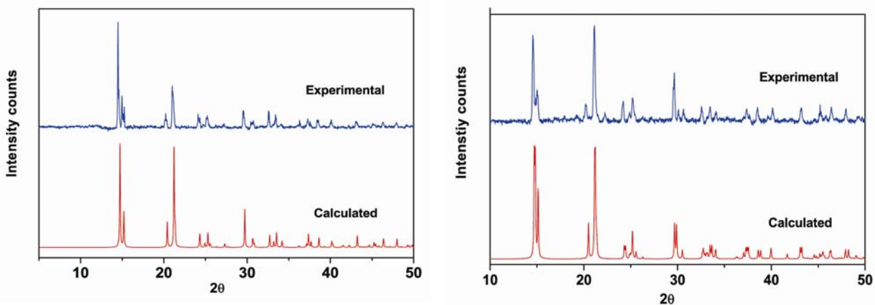
Fig. S1 Experimental and simulated XRD patterns of complexes 1a (left) and 1b (right).
