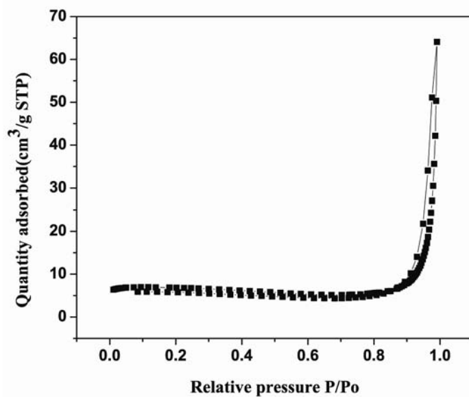
Fig. S2 N 2 adsorption and desorption plots for 1a .
