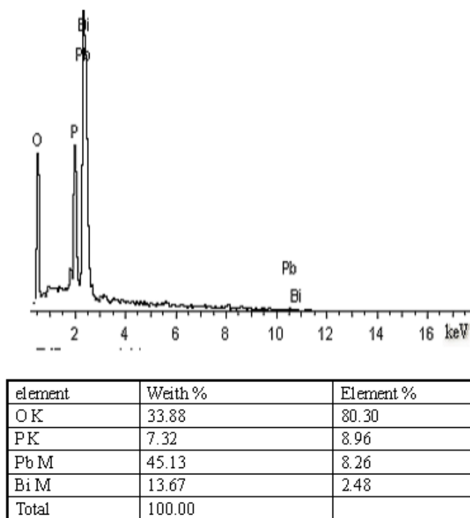
Fig. S1. EDS results of a single crystal of Pb_3BiP_3O_{12} .
