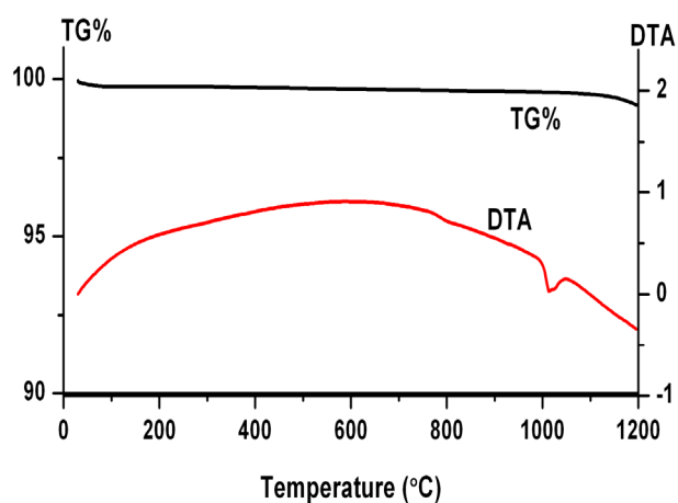
Fig. S2. TG and DTA curves for \text{Pb}_3\text{BiP}_3\text{O}_{12} .
