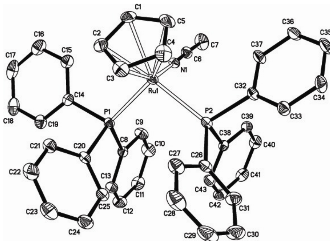
ORTEP view (30% probability) of [(\eta^5\text{-C}_5\text{H}_5)\text{Ru}(\text{PPh}_3)_2(\text{CH}_3\text{CN})]^+ ( \mathbf{M3}^+ )
