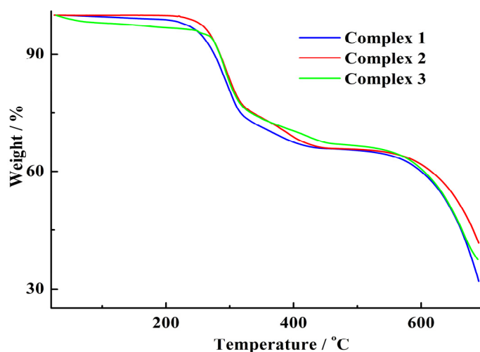
Figure S1. TGA curves for complexes 1–3.
