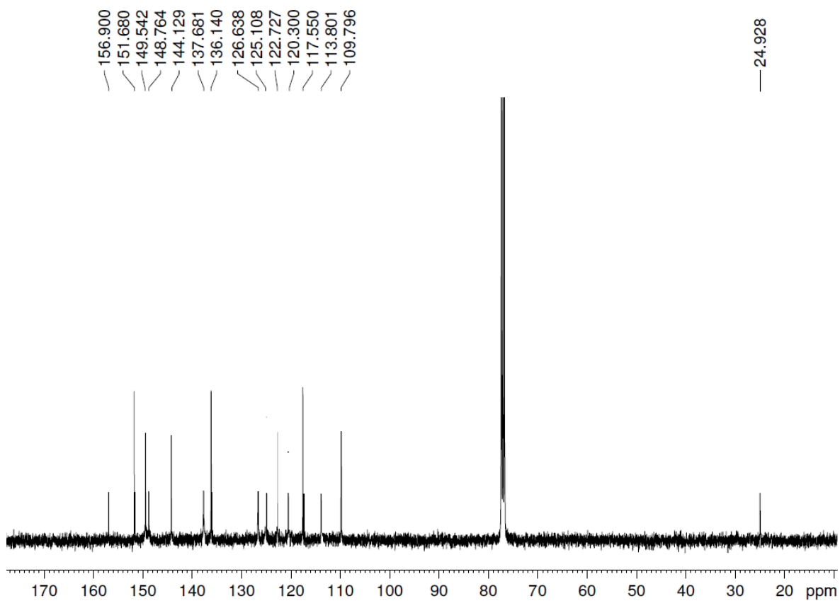
Figure S2. ^{13}\text{C} NMR spectra of 1 in chloroform
