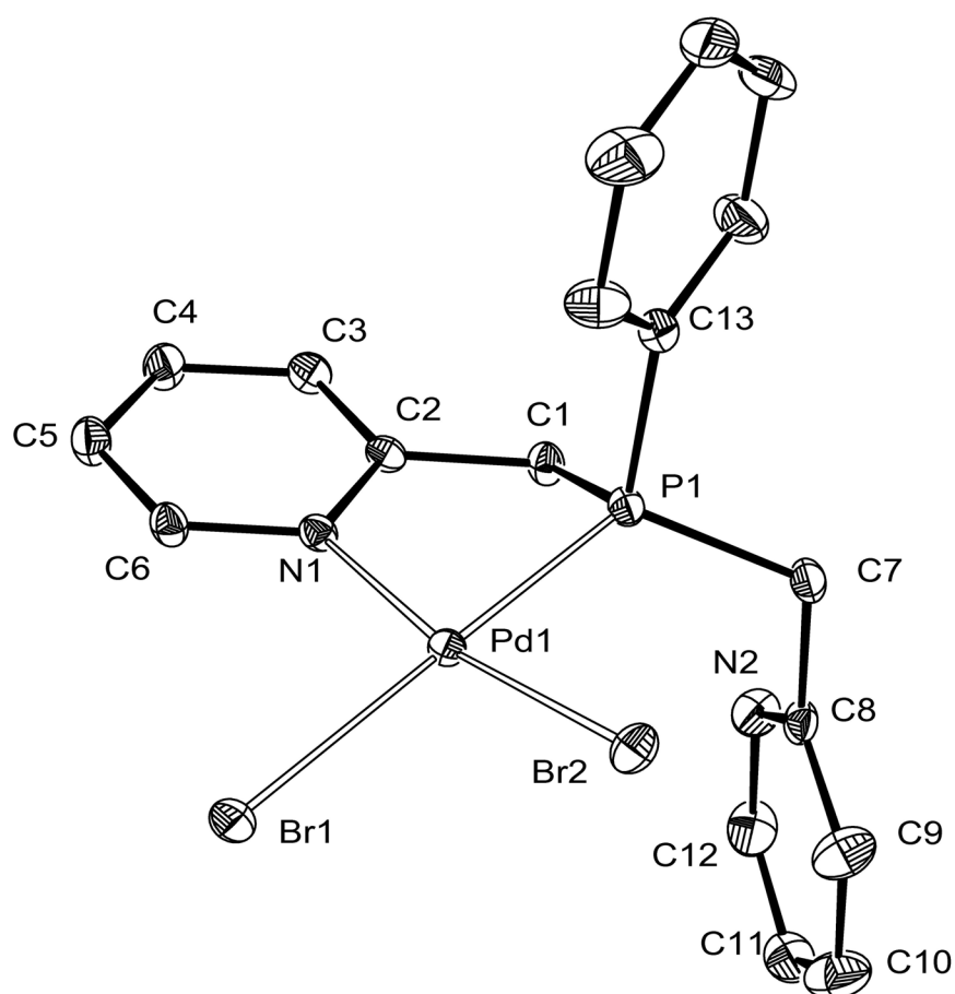
Figure S-1. ORTEP of [PdBr 2 (Npy,PNpy- N,P )] with ellipsoids drawn at the 50% probability level. Selected bond distances (Å) and angles (deg): Pd1–Br1 2.5032(5), Pd1–Br2 2.4116(5), Pd1–P1 2.2052(10), Pd1–N1 2.084(3); N1–Pd1–P1 83.31(9), N1–Pd1–Br1 96.22(8), Br1–Pd1–Br2 92.242(17), Br2–Pd1–P1 88.37(3).
