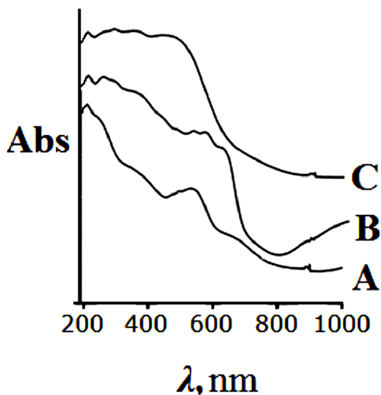
Fig. S3 UV-vis. solid state (diffuse reflectance) spectra of compounds 1(A), 2 (B) and 3·2H 2 O (C).
