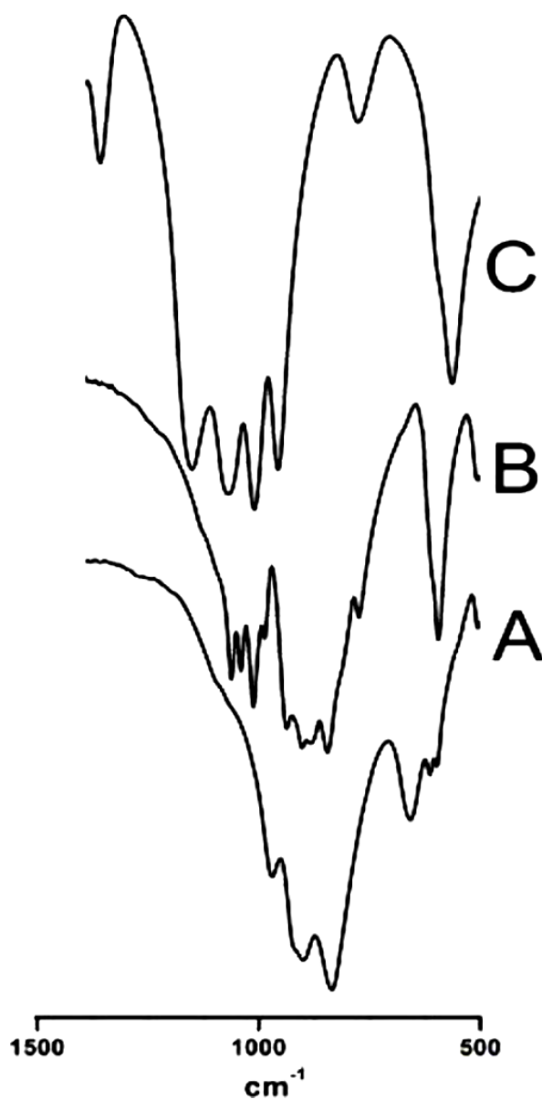
Fig. S1 Infrared spectra for compounds 1 (A), 2 (B) and 3 ·2H 2 O (C).
