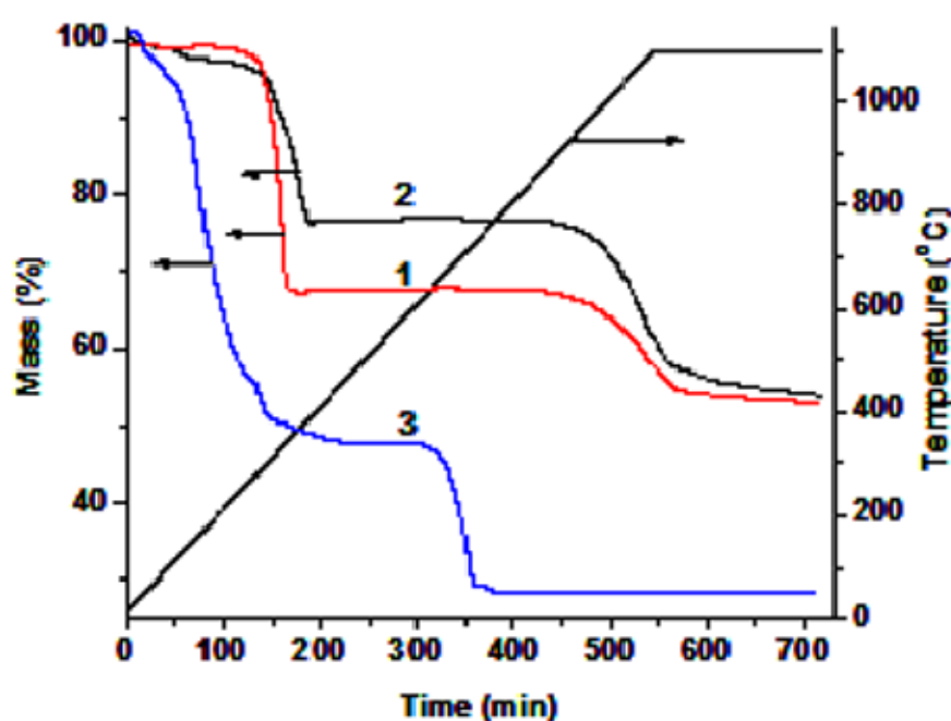
Fig. S2 Thermogravimetric curves of compounds 1, 2 and 3·2H 2 O.
