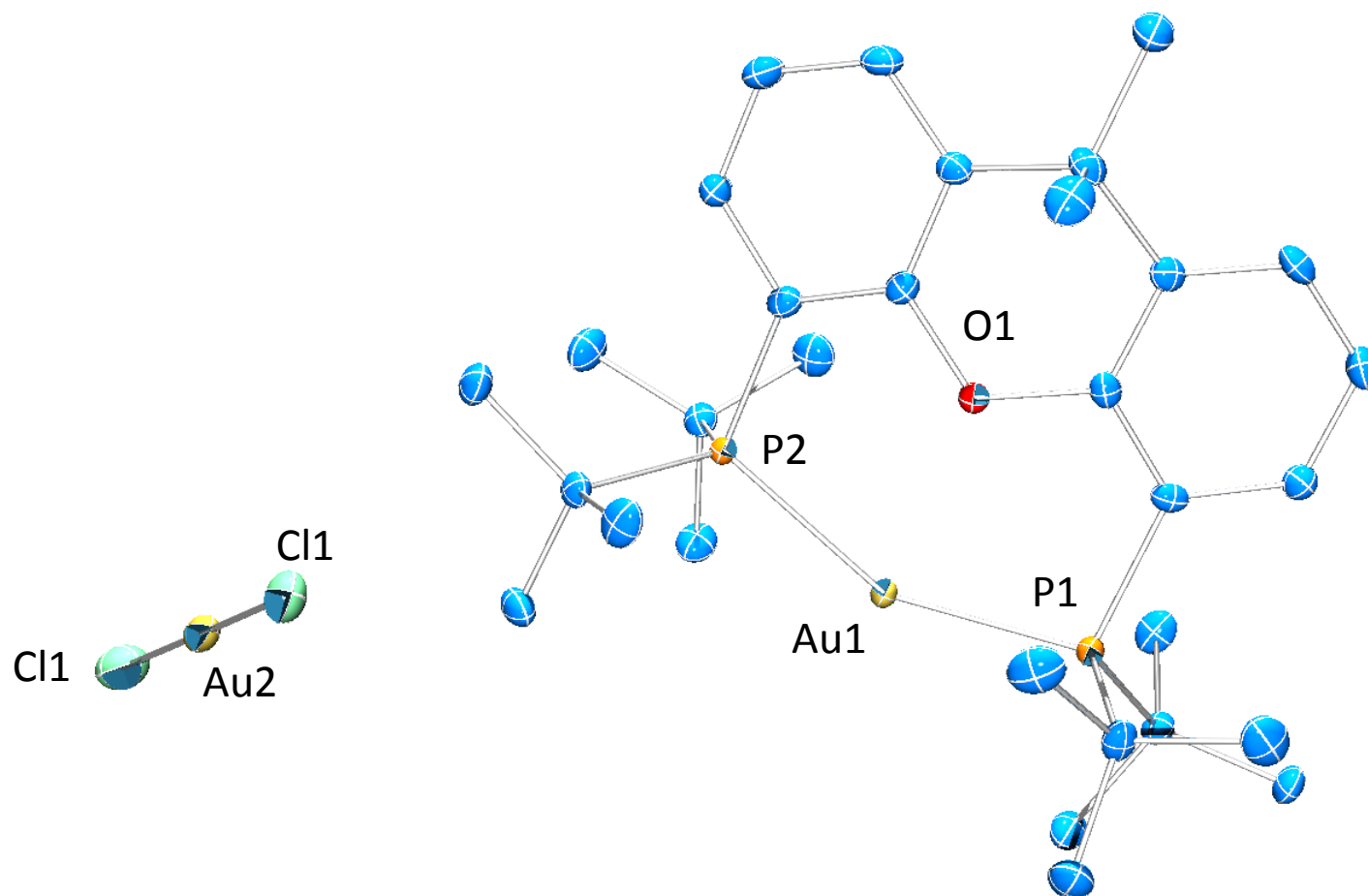
Figure S1. Thermal Ellipsoid Projection of 7 (50% probability). Unlabeled atoms are carbon; H atoms are omitted for clarity.
