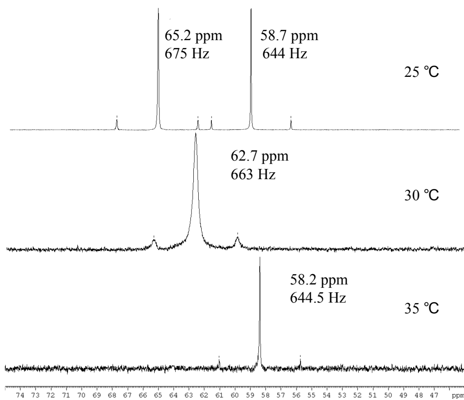
Figure S2. VT ^{31}\text{P} NMR of a mixture of compound 1 \alpha and 1 \beta .
