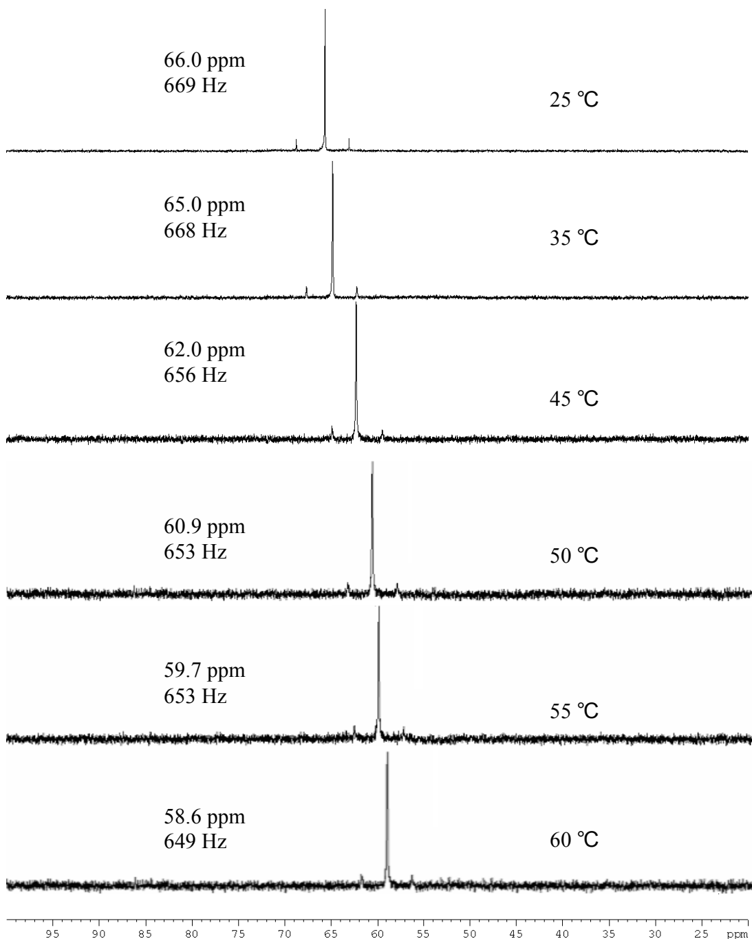
Figure S1. VT ^{31}\text{P} NMR of compound 1a .
