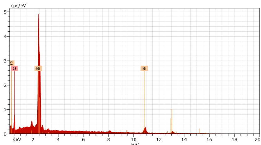
Fig. S1 The EDX spectrum of the Bi-EtOH precursor
