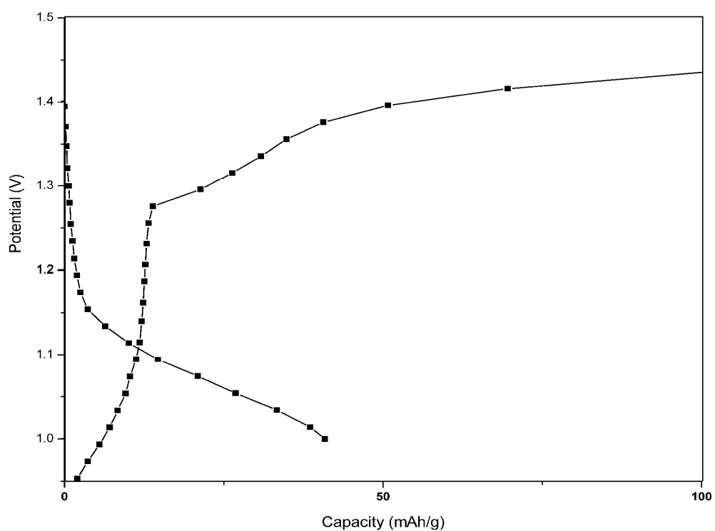
Fig. S3 The electrochemical hydrogen storage charge and discharge curve of the sample at room temperature.
