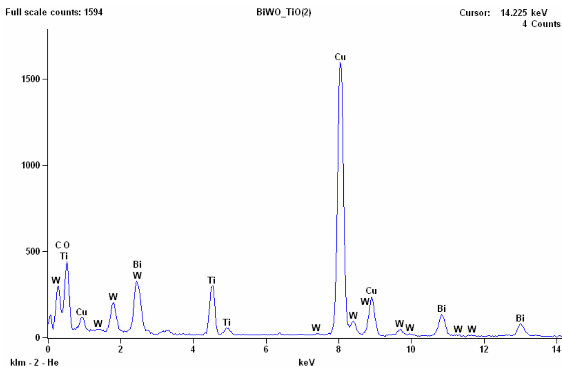
Figure S1. EDXS analysis of hierarchical \text{Bi}_2\text{WO}_6/\text{TiO}_2 composites (the Cu peak arises from the supporting Cu grid and the C peak arises from the C foil and contaminations).
