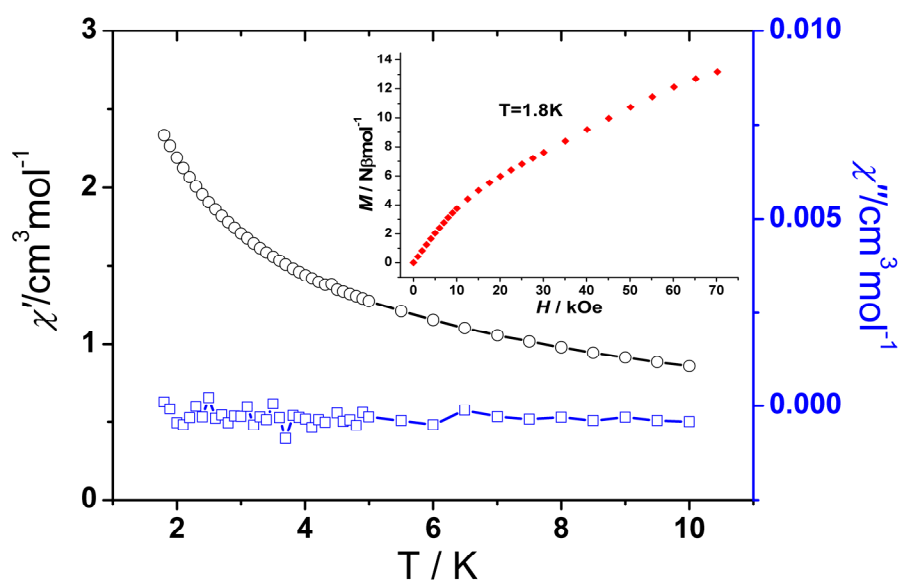
Figure S1 Real \chi' and imaginary \chi'' components of the ac susceptibility of complex I , insert for the isothermal magnetization at 1.8 K.
