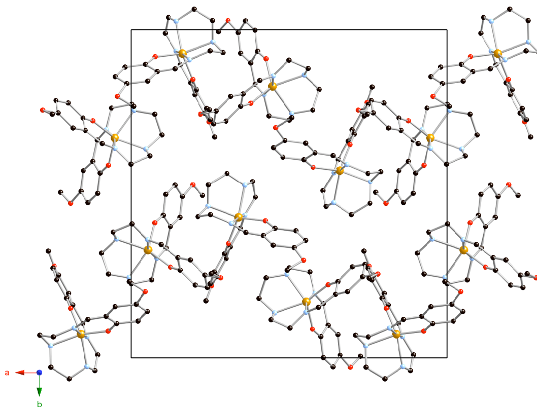
Figure S2. Projection on the ab plane of the [Fe III (5-CH 3 Osal 2 -trien)] + complexes on the structure of 2 .
