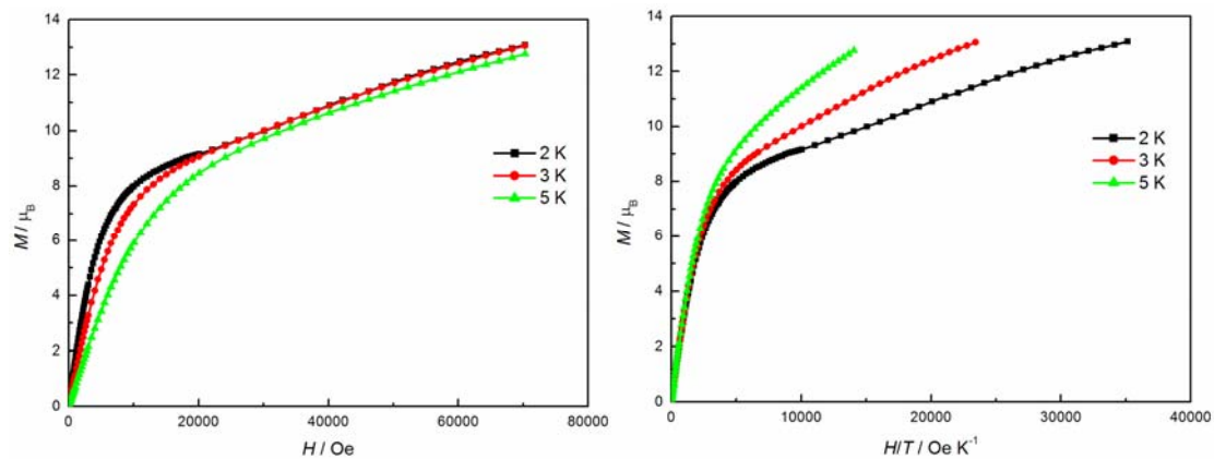
Figure S3. Field dependence of the magnetization of complex for 3.
