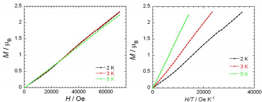
Figure S1. Field dependence of the magnetization of complex for 1.
