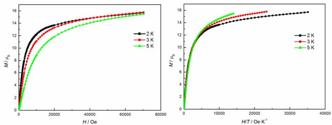
Figure S5. Field dependence of the magnetization of complex for 5.
