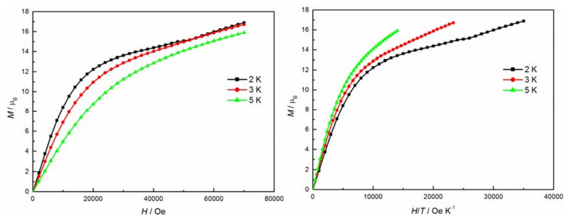
Figure S2. Field dependence of the magnetization of complex for 2.
