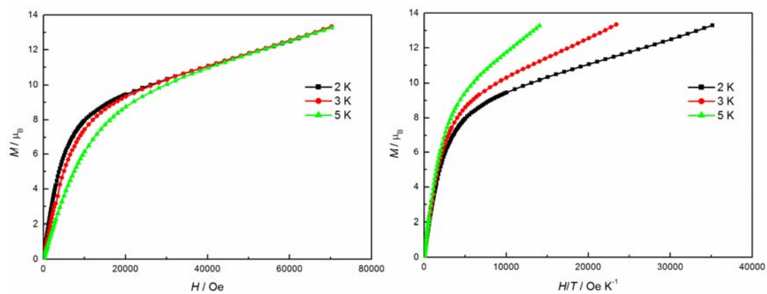
Figure S4. Field dependence of the magnetization of complex for 4.
