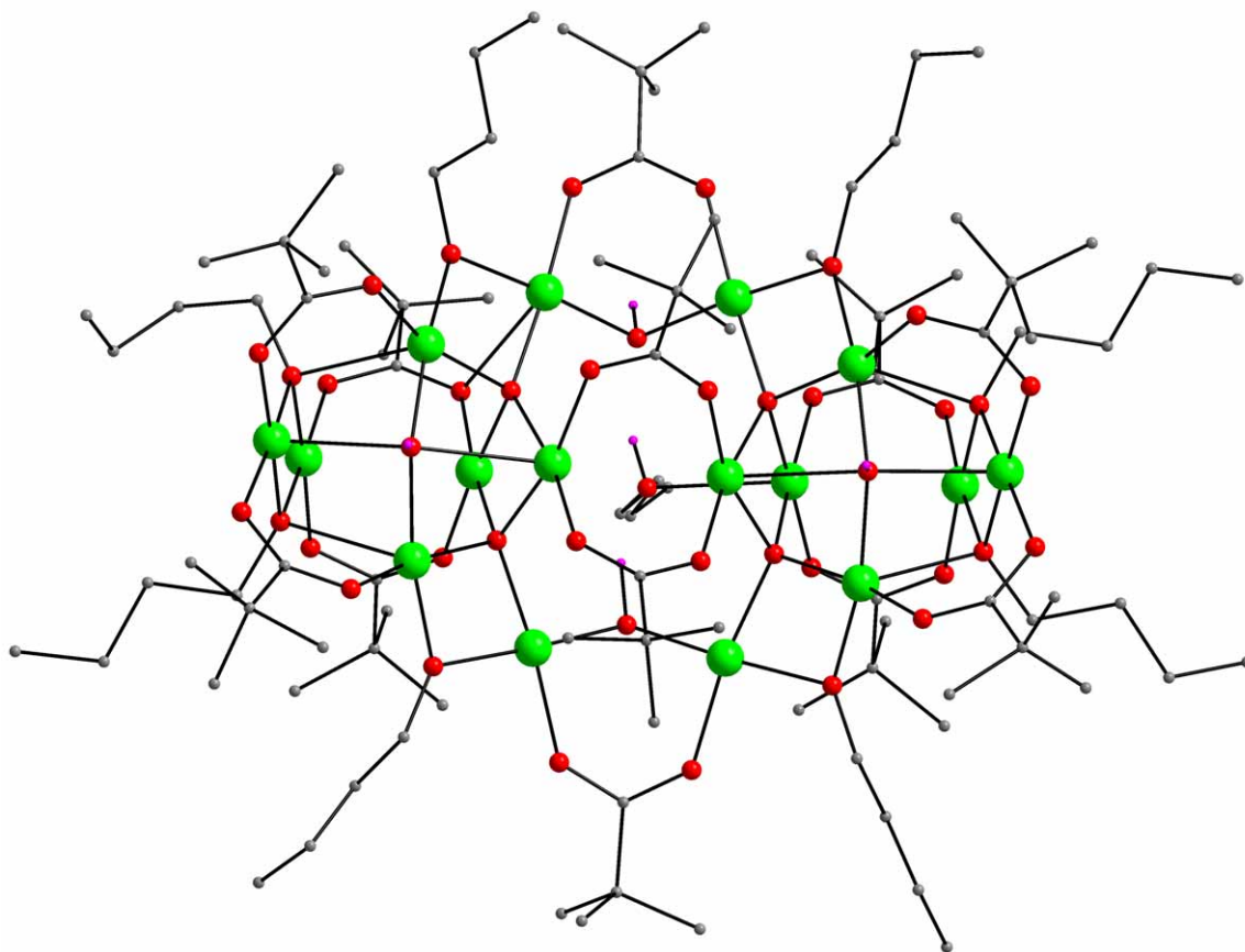
Figure S1. Molecular structure of 4 . Colour scheme: Cu II , green; O, red; C, grey; H, purple.
