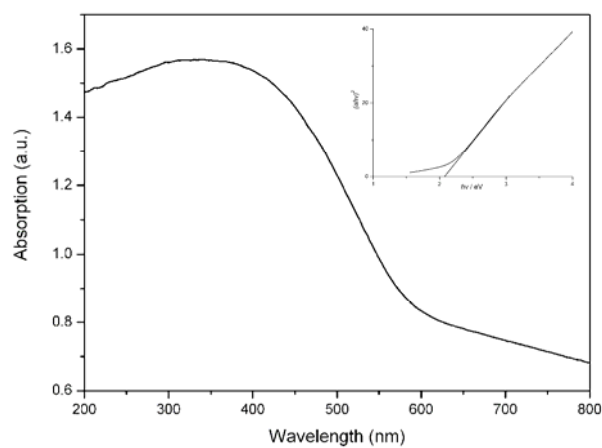
Fig, S2. The UV-Vis absorption spectrum of the sample and the corresponding calculated diagram of the band gap.
