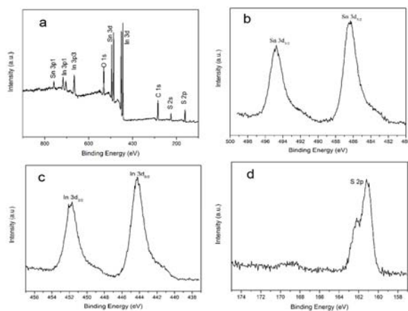
Fig. S1. a) Overall XPS spectrum of the sample. b) The high resolution spectrum of Sn 3d. c) the high resolution spectrum of In 3d. d) The high resolution spectrum of S 2p.
