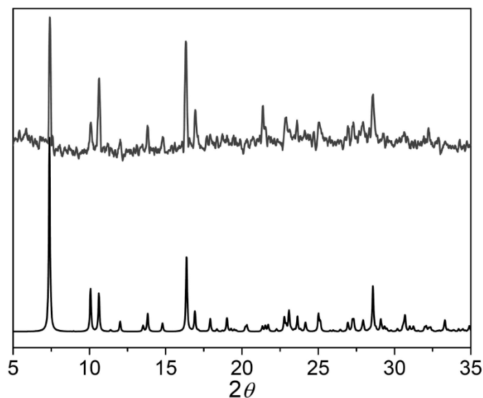
Fig. S1 Comparison of the PXRD patterns measured for 1 (gray) and that calculated from the single-crystal data of 1 (black)
