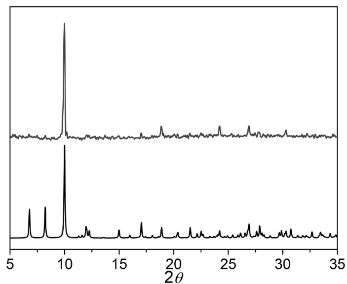
Fig. S2 Comparison of the PXRD patterns measured for 2 (gray) and that calculated from the single-crystal data of 2 (black)
