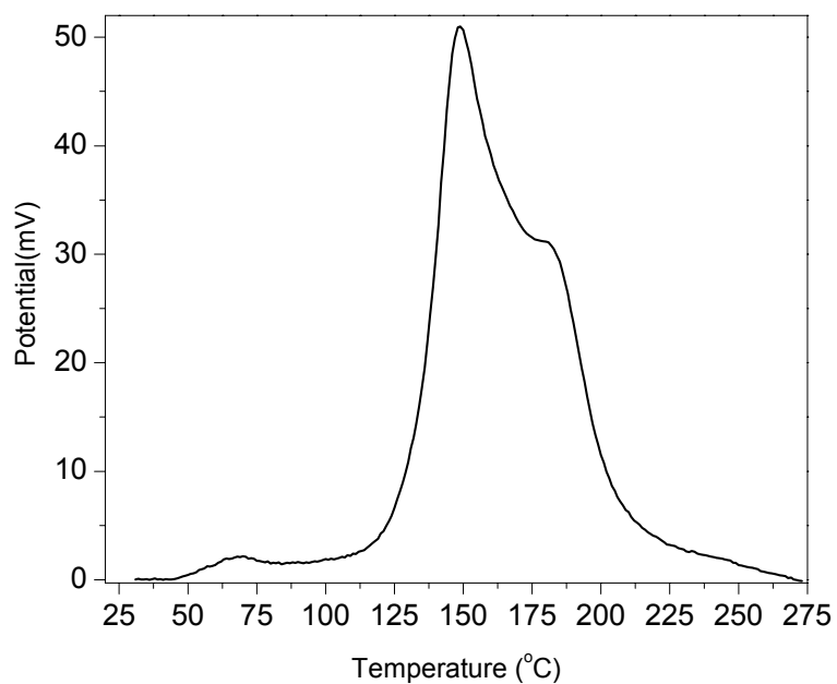
Supporting figure S2. H 2 /TPR profile of Ce 0.67 Fe 0.33 Pd 0.02 O 1.815 heated at 600 °C for 10 h.
