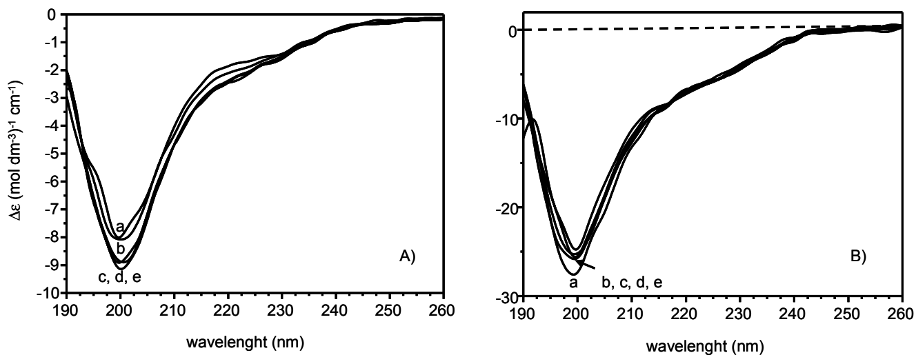
CD spectra of A) Ac-PHREN-NH 2 B) Ac-KNGNPHREN-NH 2 system, recorded in H 2 O with c(L) = 2 \times 10^{-5} \text{ mol dm}^{-3} at different pH values a) pH= 4; b) pH=6; c) pH=7; d) pH=8; e) pH=9.
