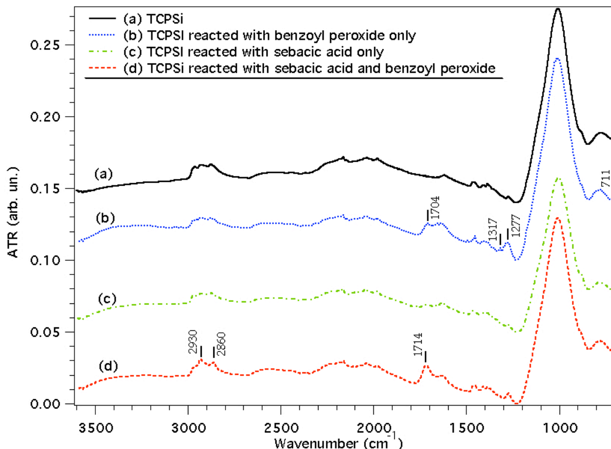
Supplemental Figure S1. Attenuated total reflectance (ATR) spectra of (a) thermally carbonized porous Si; (b) thermally carbonized porous Si chip treated with benzoyl peroxide; (c) thermally carbonized porous Si chip treated with sebacic acid only (no benzoyl peroxide); (d) thermally carbonized porous Si chip treated with sebacic acid and benzoyl peroxide.
