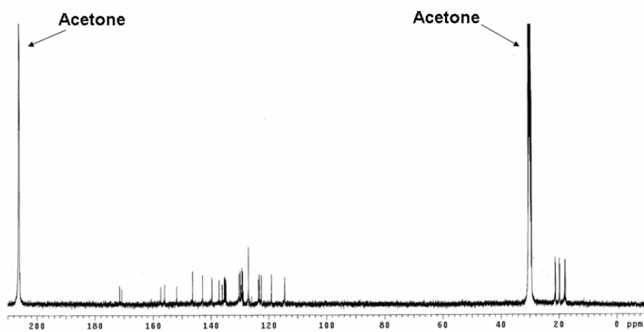
Figure S2 ^{13}\text{C} NMR spectrum of 2
