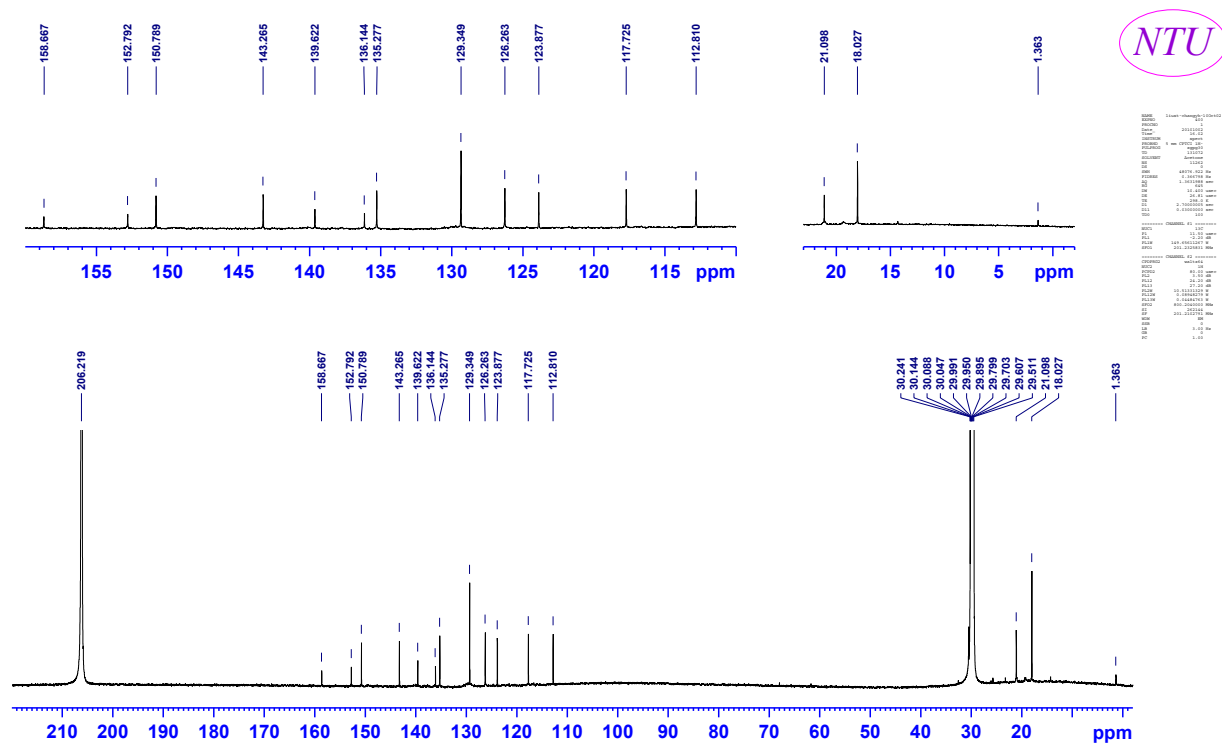
Figure S4 ^{13}\text{C} NMR spectrum of 4
