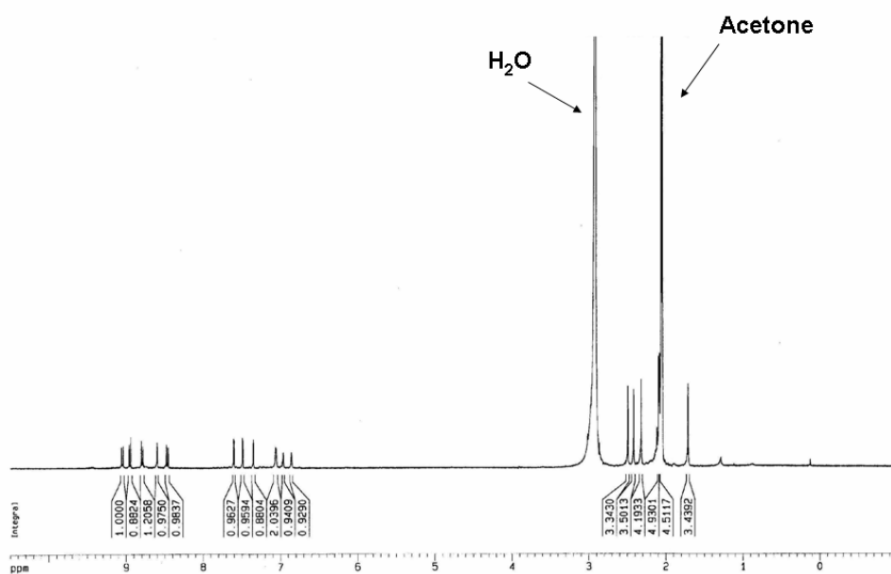
Figure S1 ^1\text{H} NMR spectrum of 2
