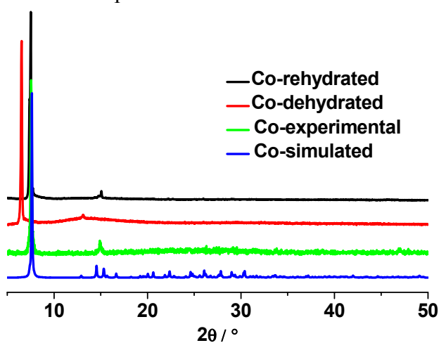
Figure S3. XRD patterns for as-synthesized, the dehydrated and rehydrated compound 1.
