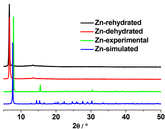
Figure S4. XRD patterns for as-synthesized, the dehydrated and rehydrated compound 2.
