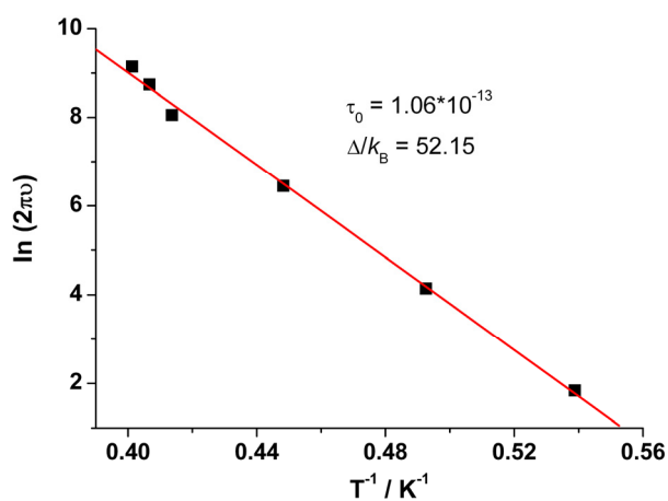
Figure S6. Plot of \ln(2\pi\nu) versus reciprocal temperature for 1-de .
