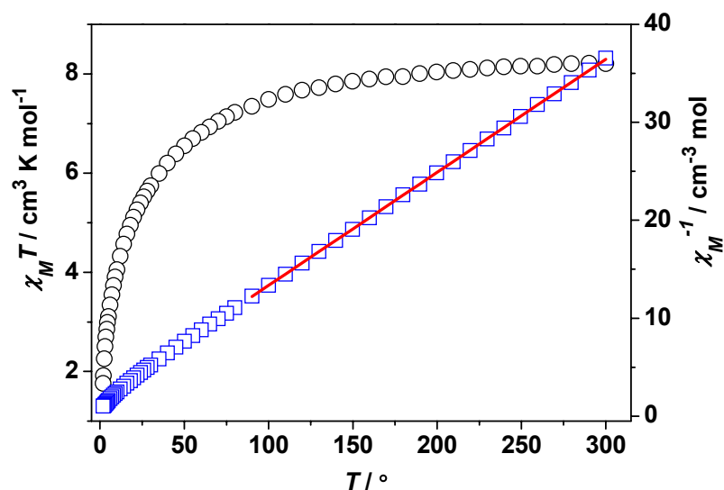
Figure S5. The \chi_M^{-1} and \chi_M T vs T plots for the 1-de .
