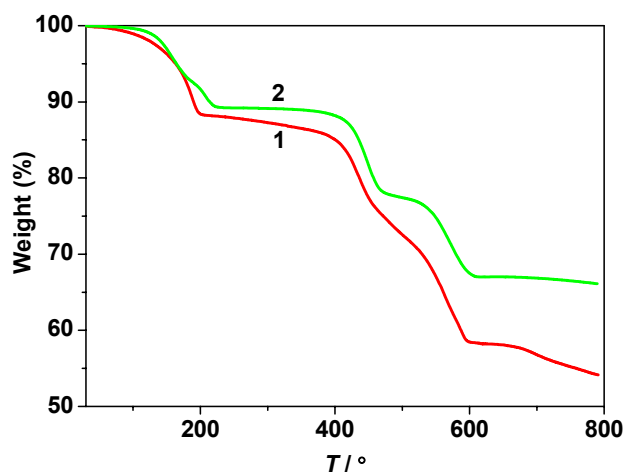
Figure S2. TGA curves for compounds 1 and 2.
