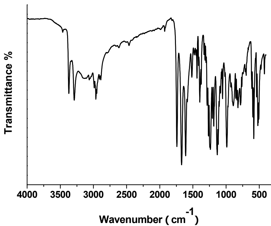
Fig.S2 The infrared spectrum of the complex 2
