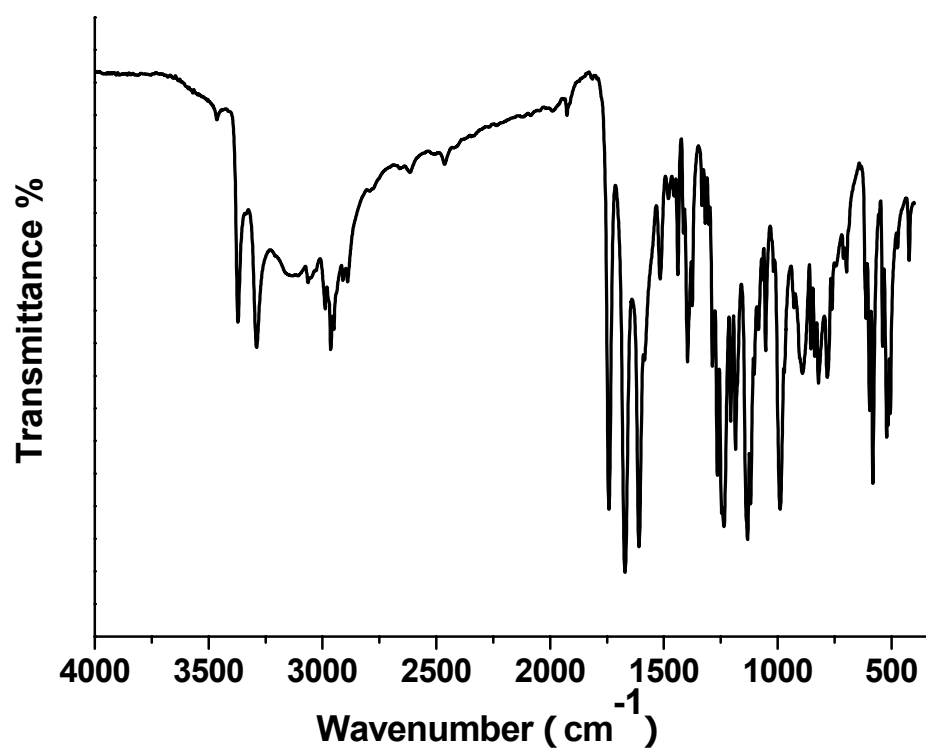
Fig.S1 The infrared spectrum of the complex 1
