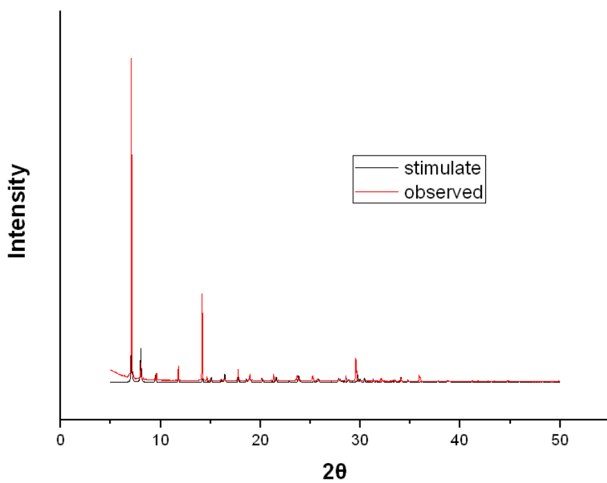
Fig.S6 PXR D of the complex 3
