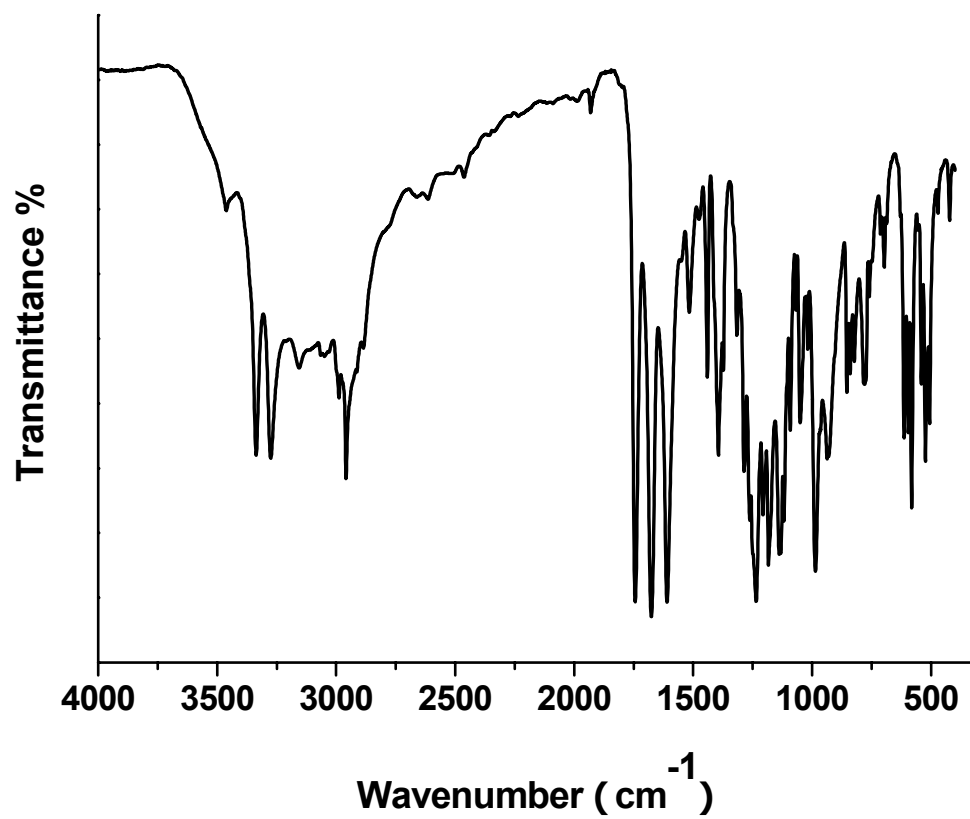
Fig.S3 The infrared spectrum of the complex 3
