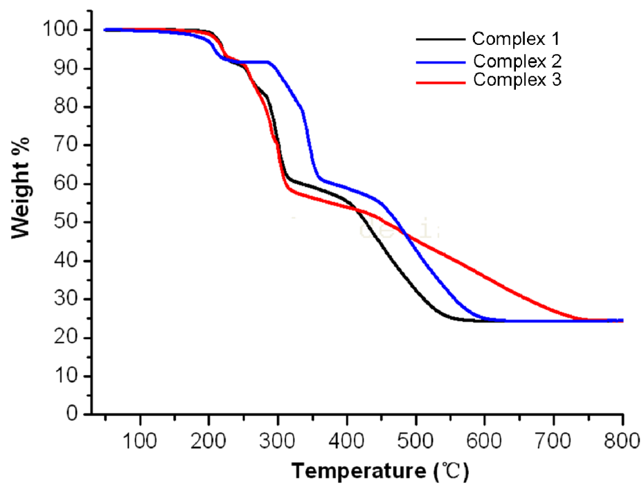
Fig.S7 TG curves of complex 1, complex 2, and complex 3
