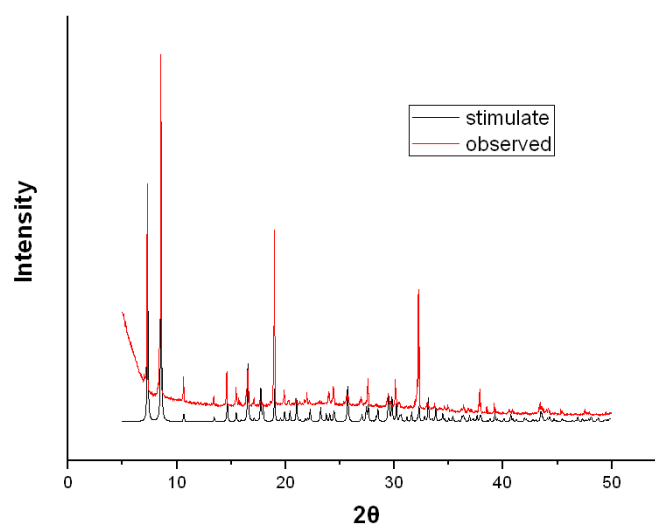
Fig.S4 PXRD of the complex 1
