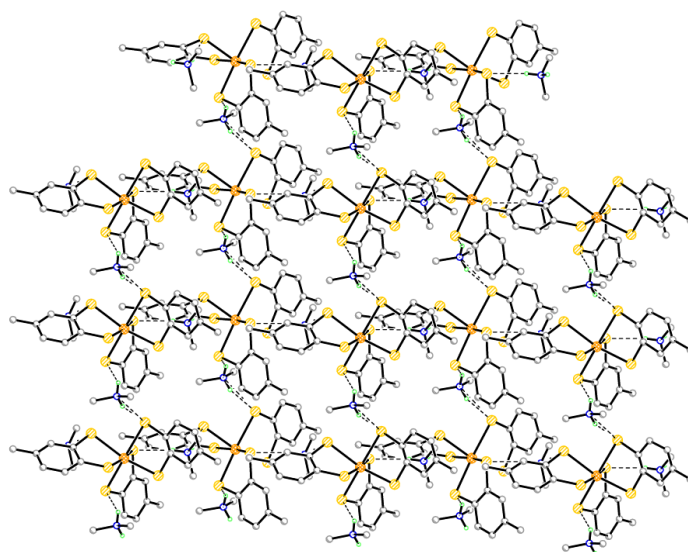
Fig. S3 Packing of ions in the lattice of 3 . Range S \cdots H 2.24-2.47Å.
