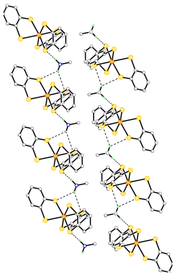
Fig. S2 Packing of ions in the lattice of 3 . Range S...H 2.52-2.82 Å.
