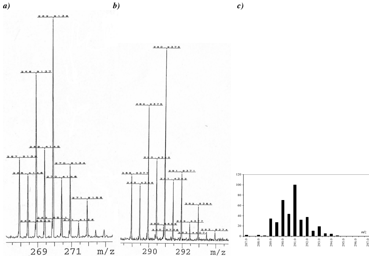
Fig. S1 Negative-ion Mass Spectrum of a) 2 and b) 3 , showing the dianion envelope, and c) the calculated spectrum for 3 .
