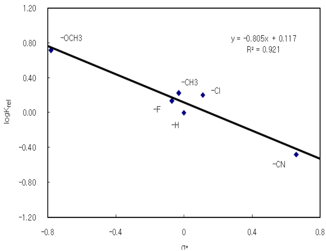
Fig. S1 Hammett plot for relative reactivities of styrene to para -substituted styrenes with 6 .
