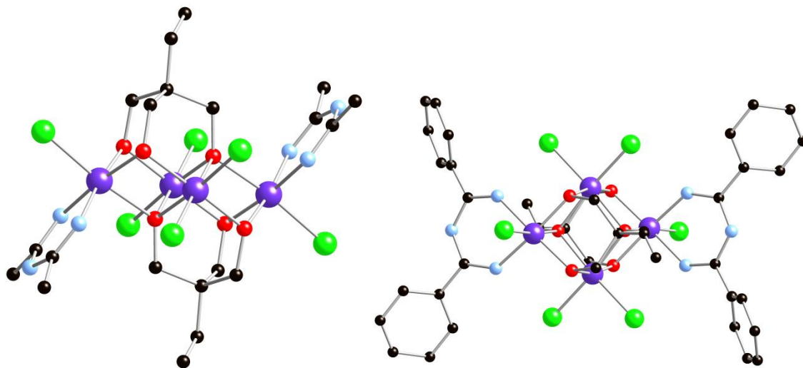
Figure S2. Views of the structures of complexes 5 (left) and 7 (right). Scheme as in Fig. 1.
