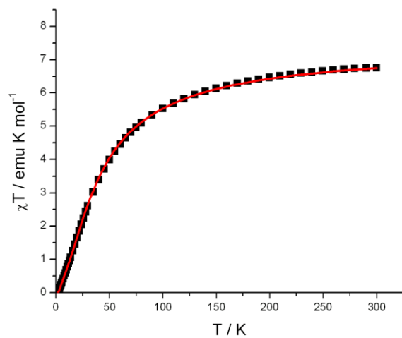
Figure S4. \chi T(T) for 7 in an applied field of 1.0 T: experimental (data points) and calculated (red line).
