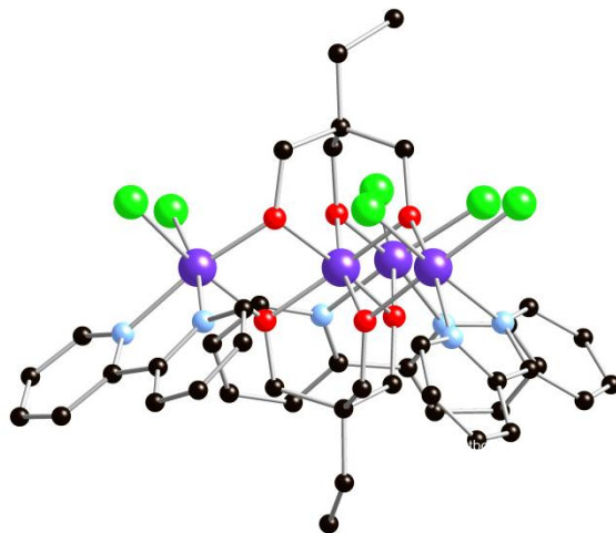
Figure S1. Structure of complex 2 viewed in the {Cr 4 } plane. Scheme as in Fig. 1.
