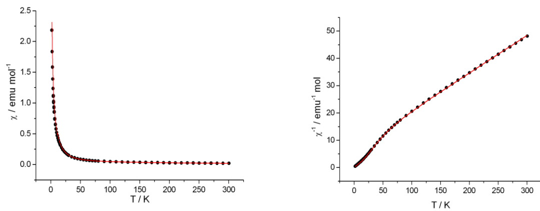
Figure S3. \chi(T) (left) and \chi^{-1}(T) (right) for 2 : experimental (data points) and calculated (red lines).
