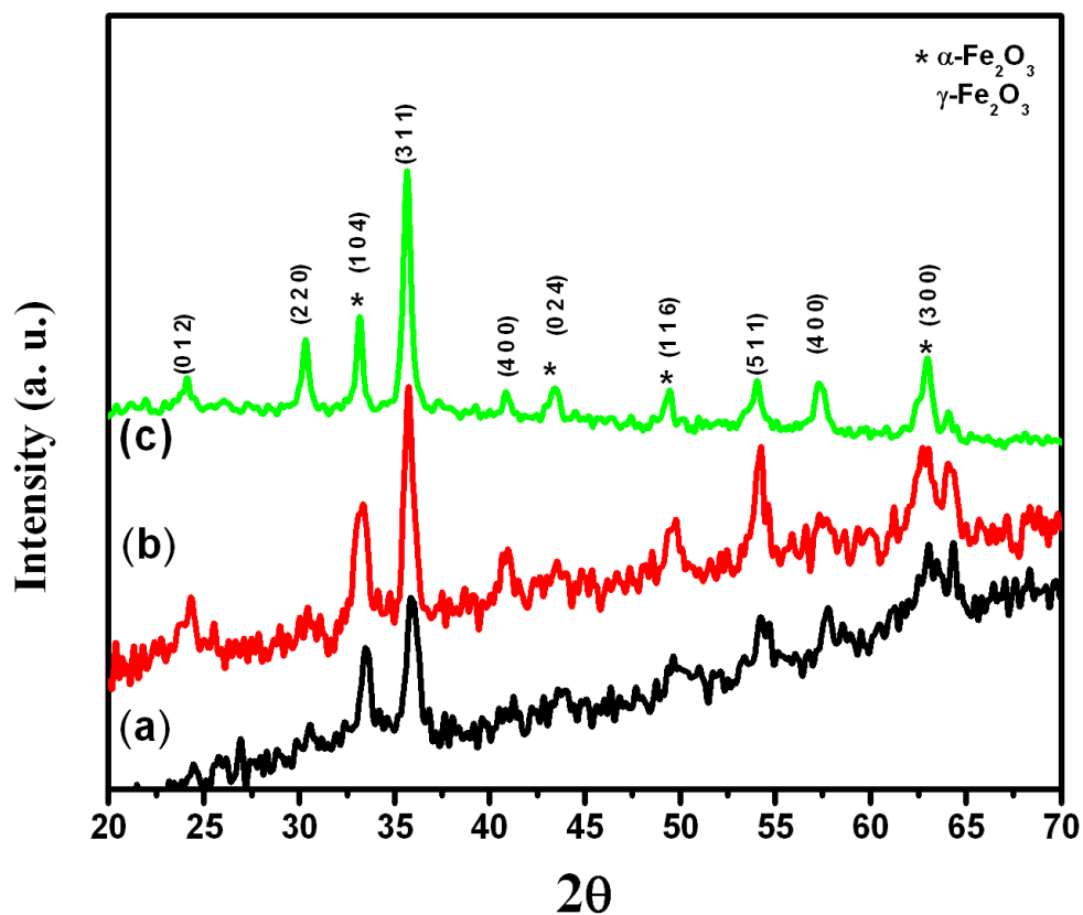
Fig. SI-1 XRD spectra of Fe-complex annealed at 450 °C for 180 min with different heating rate (a) 1 °C, (b) 10 °C and (c) 15 °C
