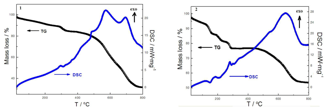
Fig. S3 TG-DSC curves of 1 and 2 .
