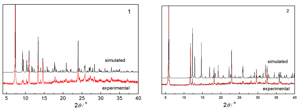
Fig. S2 The powder XRD patterns of 1 and 2 .
