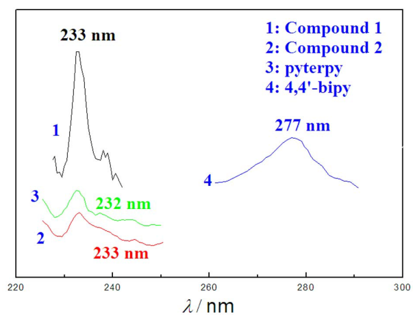
Fig. S4 Excitation spectra of different compounds.
