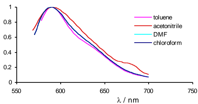
Figure S3. Emission spectra of 7 in different solvents (ca. 10^{-5} M) at room temperature.
