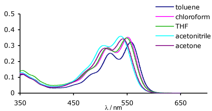
Figure S2. Absorption spectra of 7 in different solvents (ca. 10^{-5} M) at room temperature.
