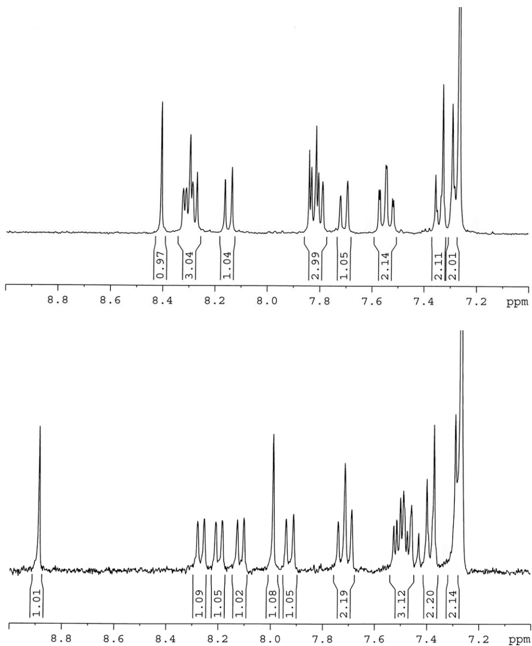
Figura S1. 1 H NMR spectra (aromatic hydrogen atoms) for the xanthate complexes 3 (top) and 8 (bottom).
