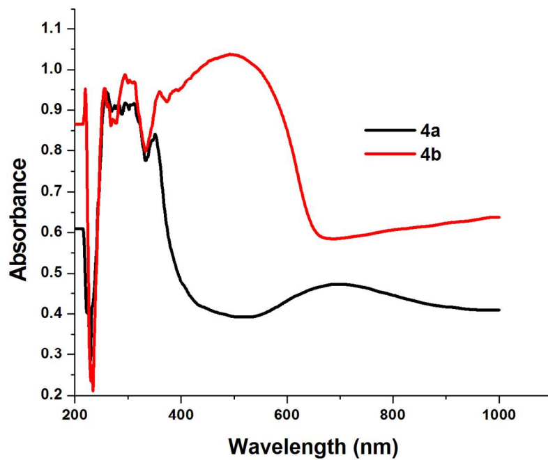
Figure S5. Absorption spectra of 4a and 4b in solid state.
