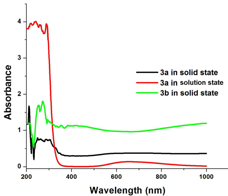
Figure S4. Absorption spectra of 3a and 3b .
