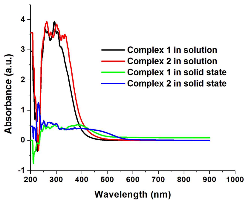
Figure S3. Absorption spectra of 1 and 2 .
