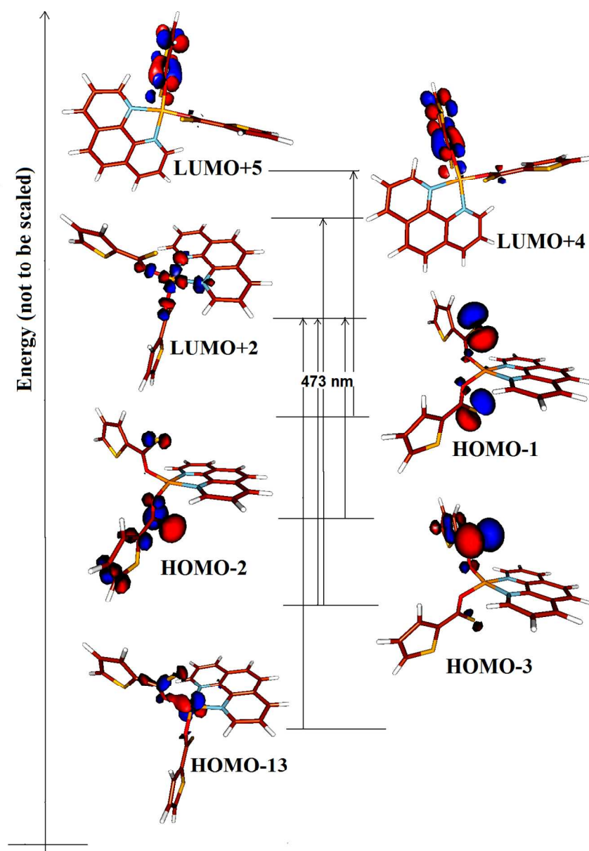
Figure S6. Selected transitions in 4a (orbital contour value = 0.05)
