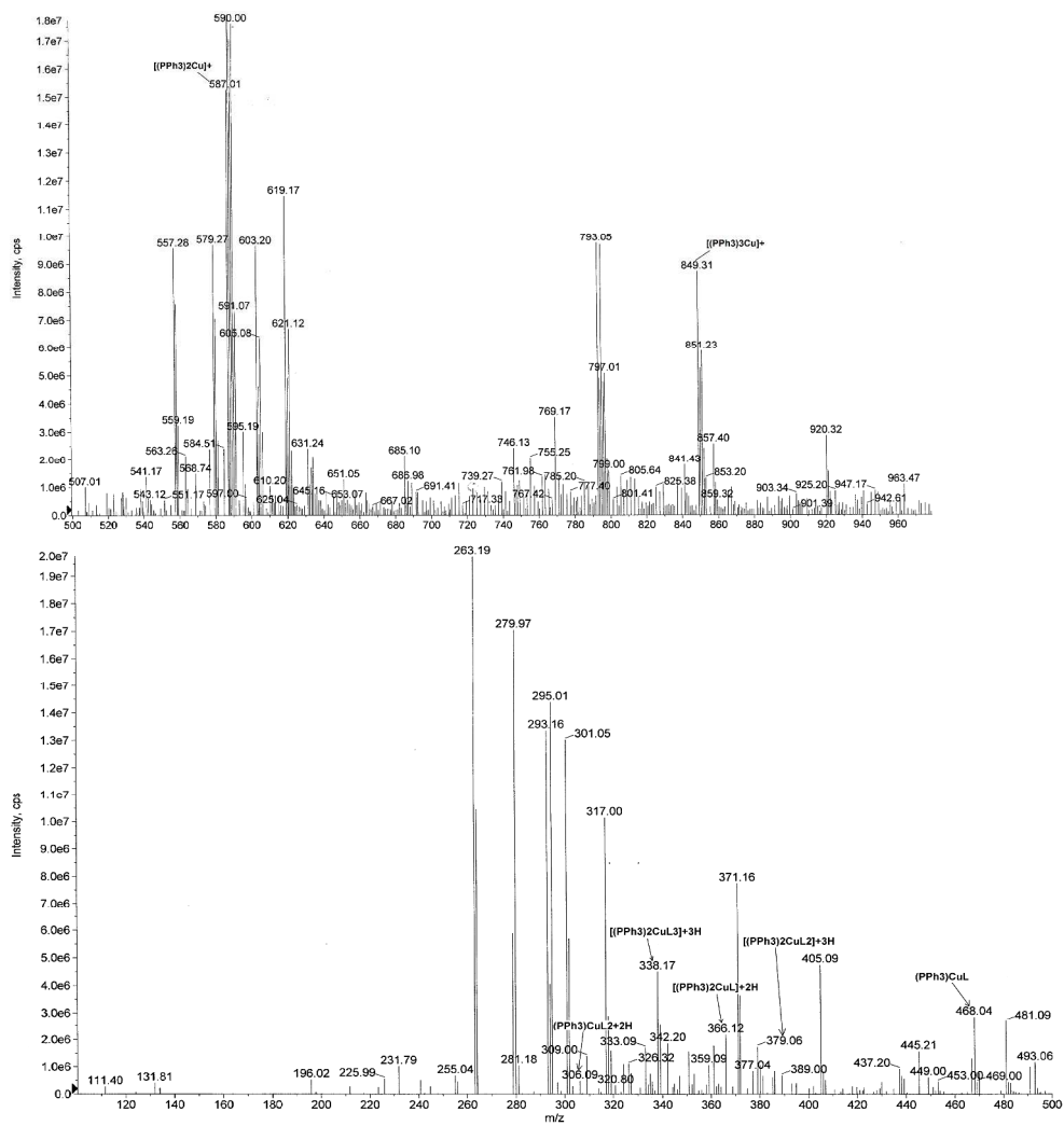
Figure S1. ES-Mass spectrum of 1
