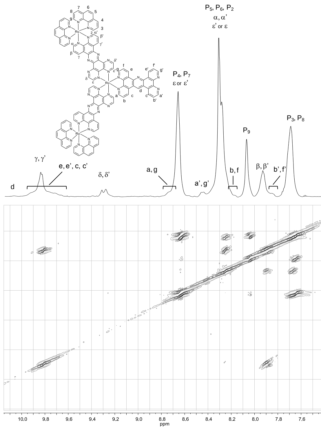
Figure S2. ^1\text{H} NMR spectra for complex 5 obtained in \text{CD}_3\text{CN} at 600 MHz.
