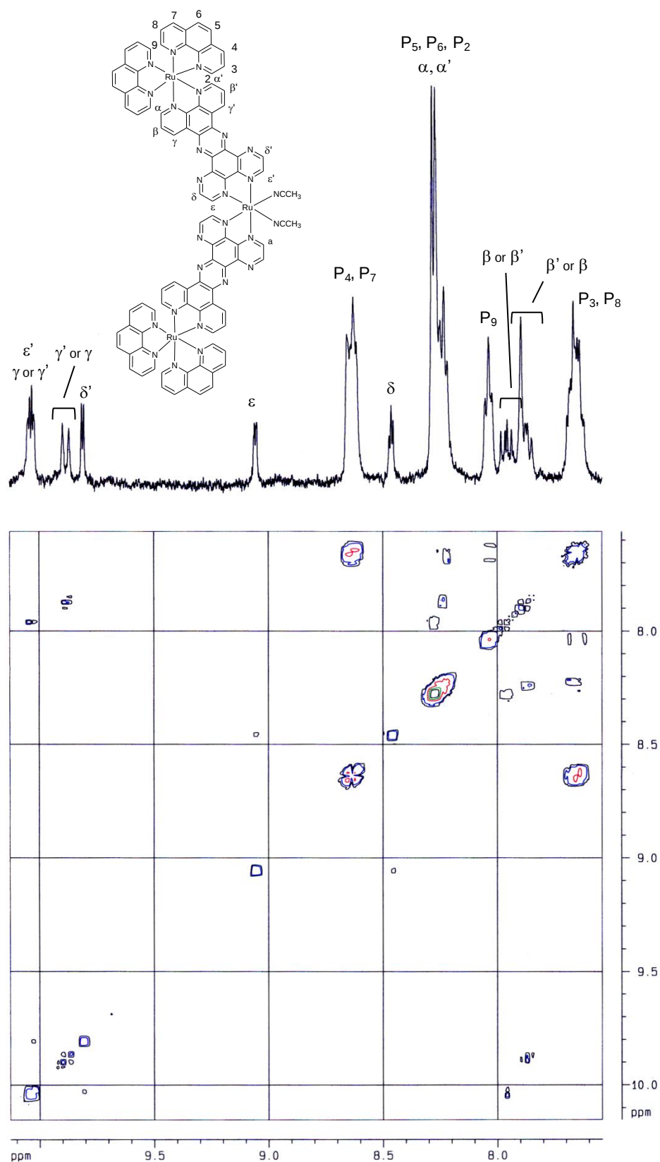
Figure S1. ^1\text{H} NMR spectra for complex 4 obtained in \text{CD}_3\text{CN} at 300 MHz.
