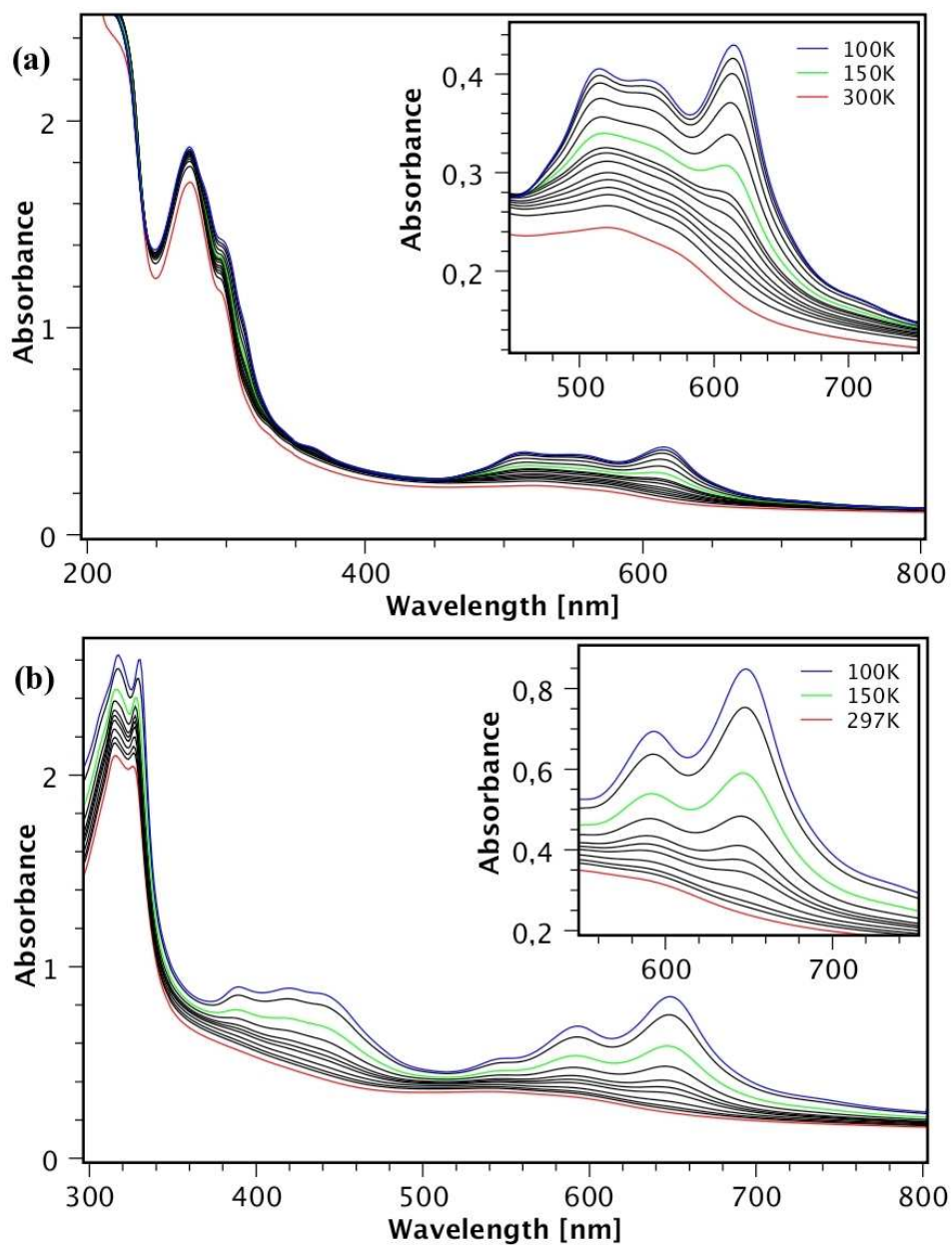
Fig. S2 UV/Vis Spectra of KBr pellets of 1 and 2.
