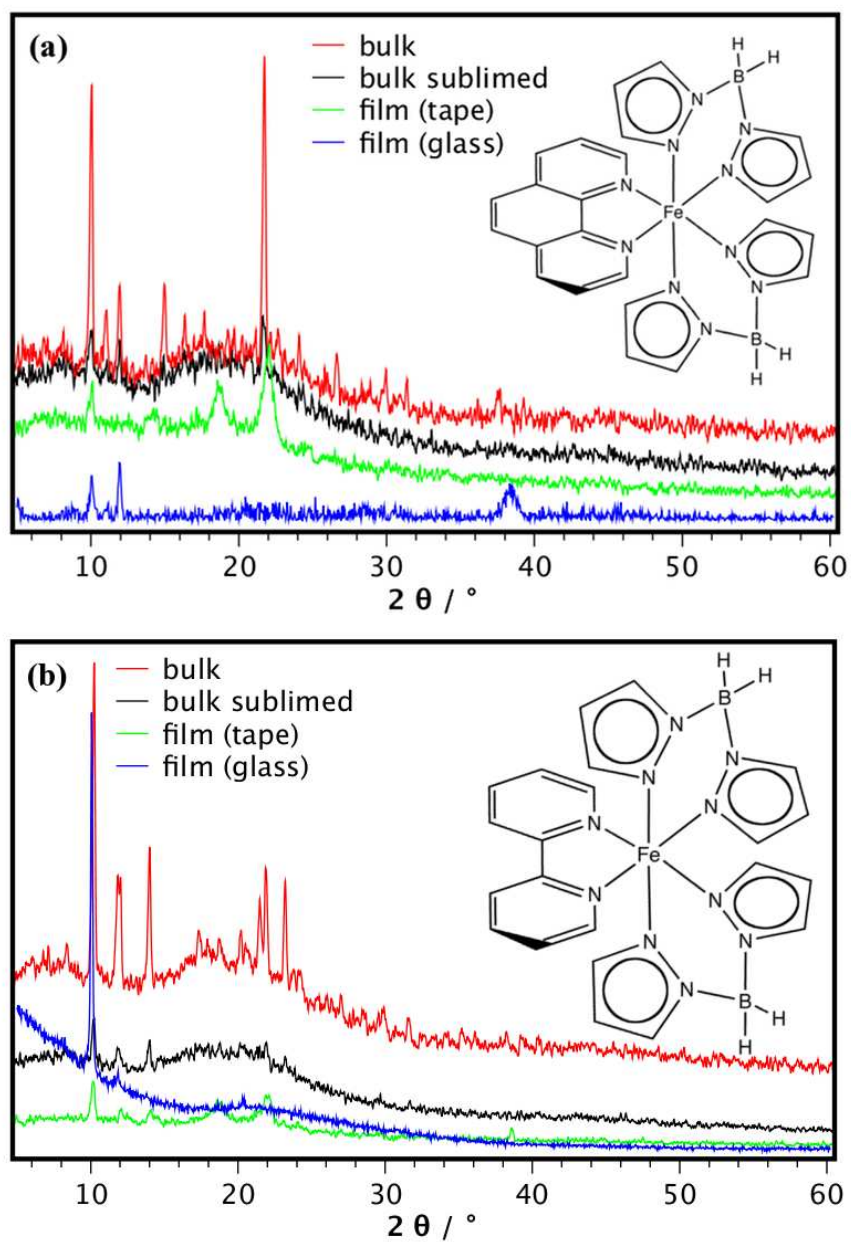
Fig. S1 X-ray-diffractograms of bulk, sublimed bulk, film on tape and film on glas for 1 and 2.
