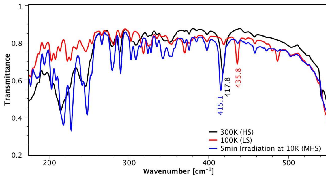
Fig. S3 FIR Spectra of a thin film of 2 at 300 and 10 K.
