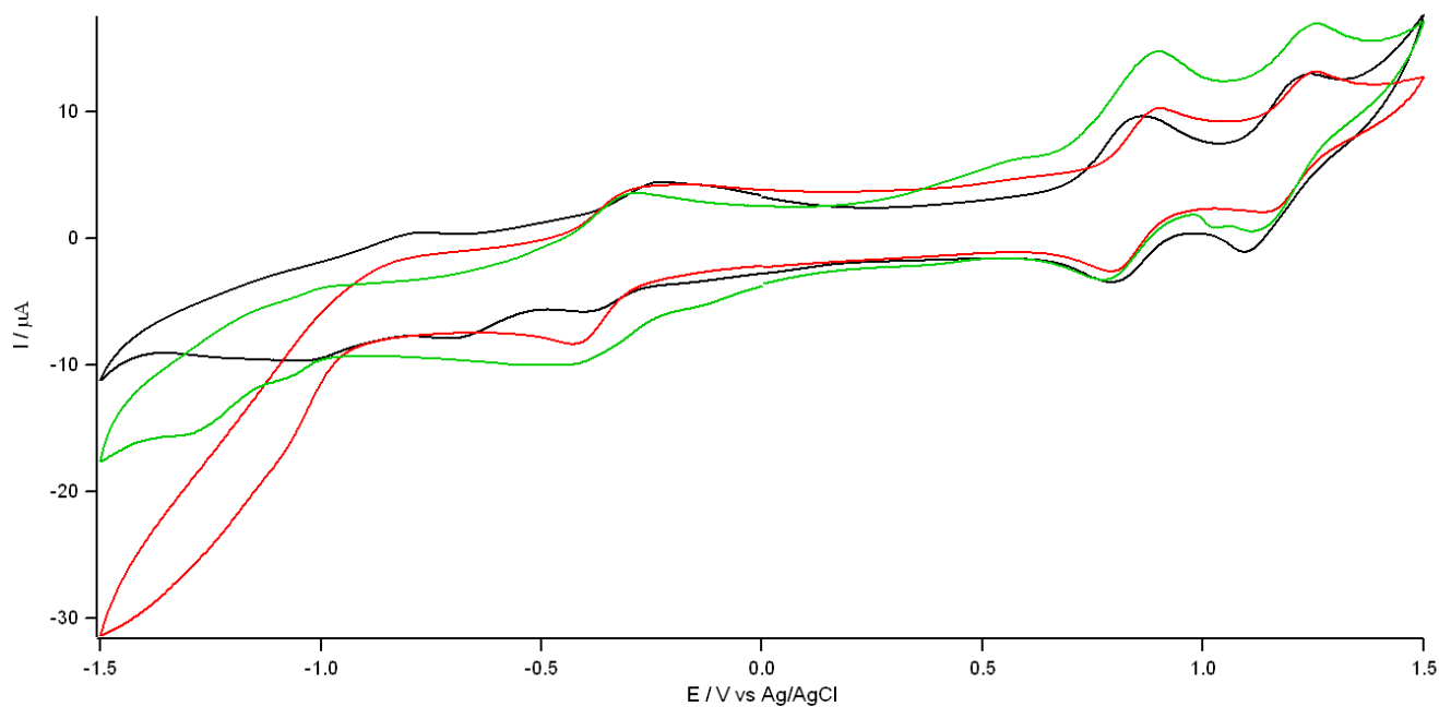
Figure S4. Cyclic voltammograms of 1 ( 5 \times 10^{-4} M, black), 2 ( 5 \times 10^{-4} M, red) and 3 ( 5 \times 10^{-4} M, green) in \text{CH}_2\text{Cl}_2 (0.1 M TBAPF 6 ; platinum working electrode; scan rate 100 \text{ mV} \cdot \text{s}^{-1} ).
