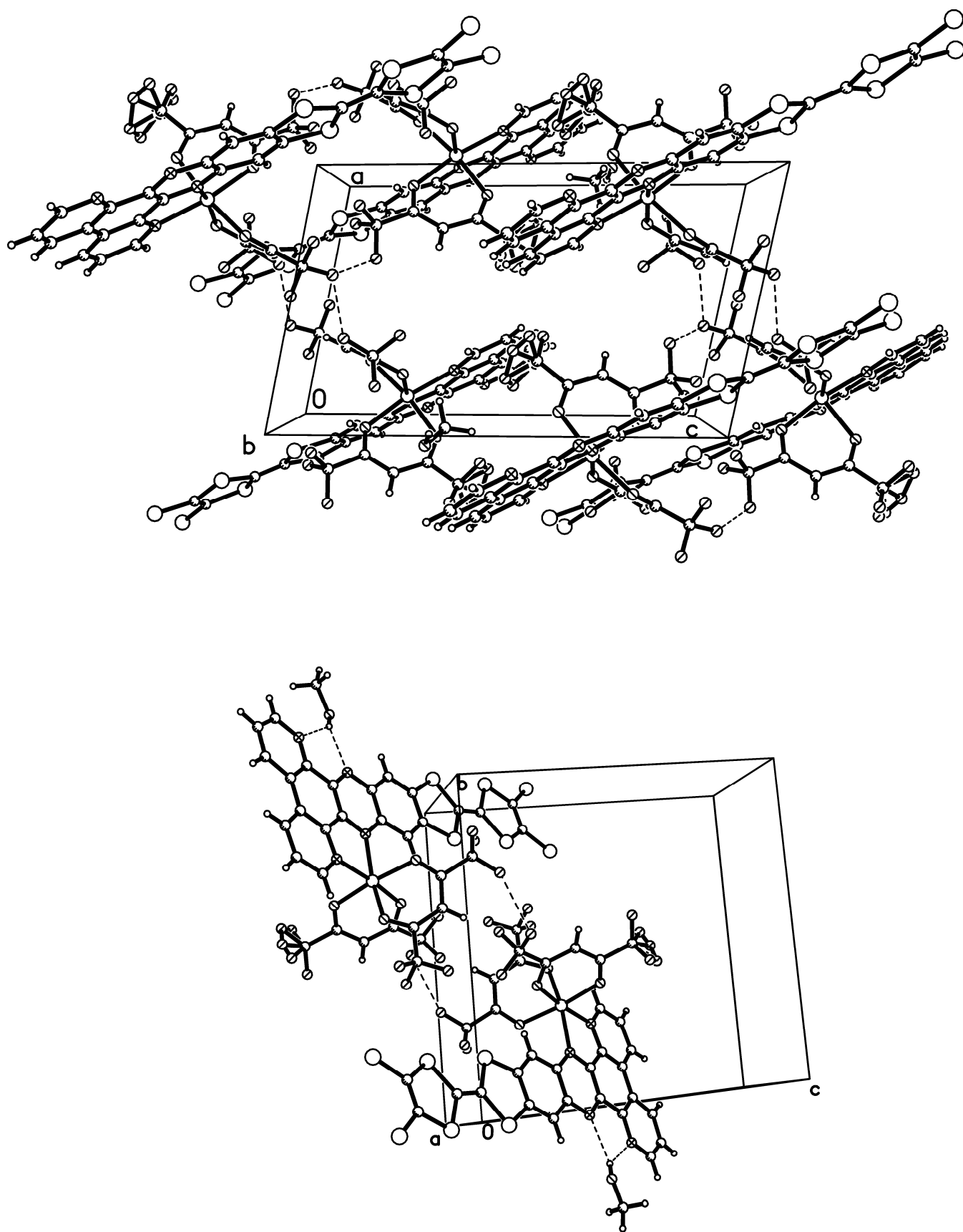
Figure S2. Crystal packing diagram of 1 , showing some intermolecular hydrogen bonds O-H...N and F...F close contacts. The n-propyl groups of the TTF-PPB ligand are omitted for clarity.
