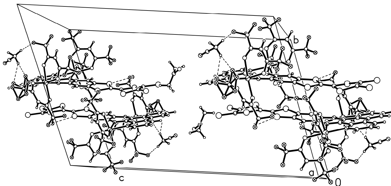
Figure S3. Crystal packing diagram of 2 , showing a head-to-tail arrangement through some short contacts. The n-propyl groups of the TTF-PPB ligand are omitted for clarity.
