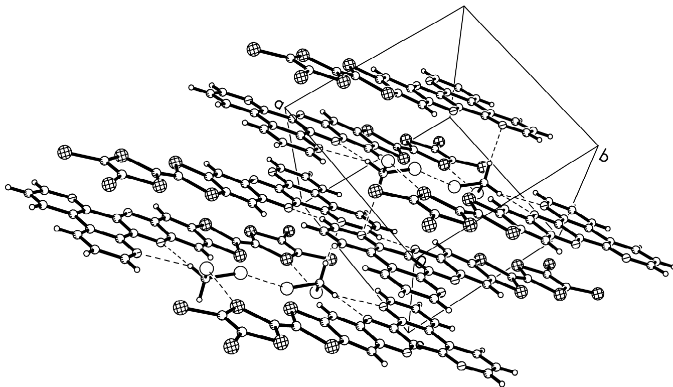
Figure S1. Crystal packing diagram of the bridging ligand TTF-PPB with the highlight of intermolecular hydrogen bonds C-H...N and some selected close contacts. The n-propyl groups of the TTF-PPB ligand are omitted for clarity.
