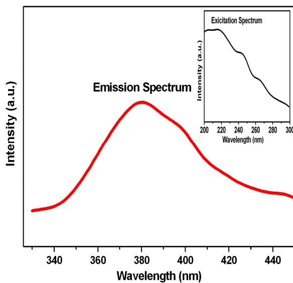
Fig. S4 Solid-state emission spectrum of complex 3 at room temperature.
