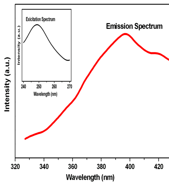
Fig. S3 Solid-state emission spectrum of complex 2 at room temperature.
