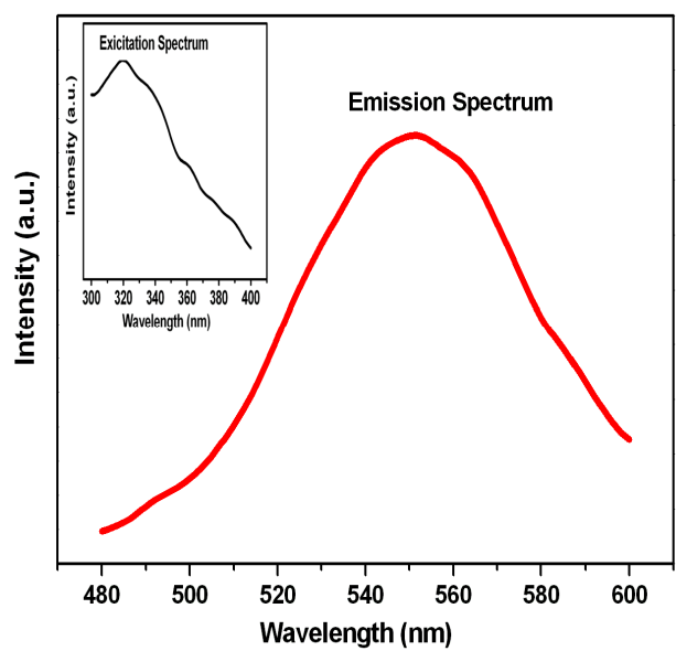
Fig. S5 Solid–state emission spectrum of complex 4 at room temperature.
