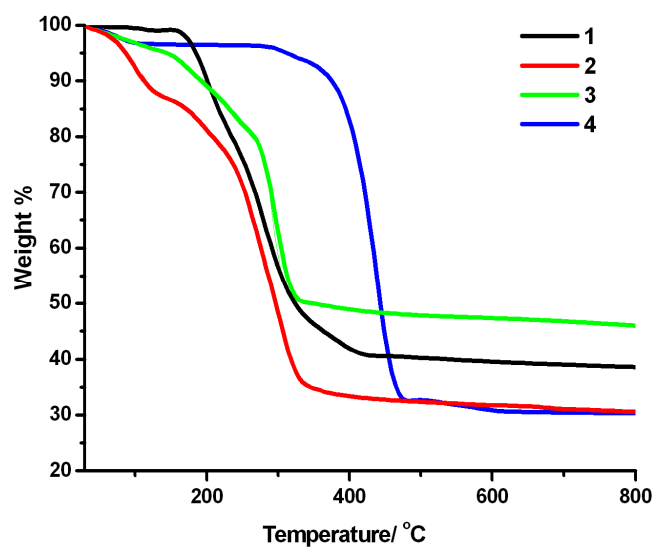
Fig. S1 TG curves for compounds 1–4.
