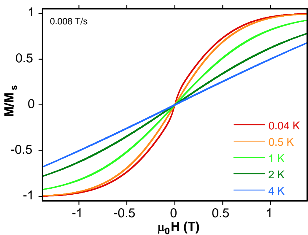
Figure S1. Magnetization vs. field plot for complex 1 at 0.008 T/s scan rate and several temperatures.
