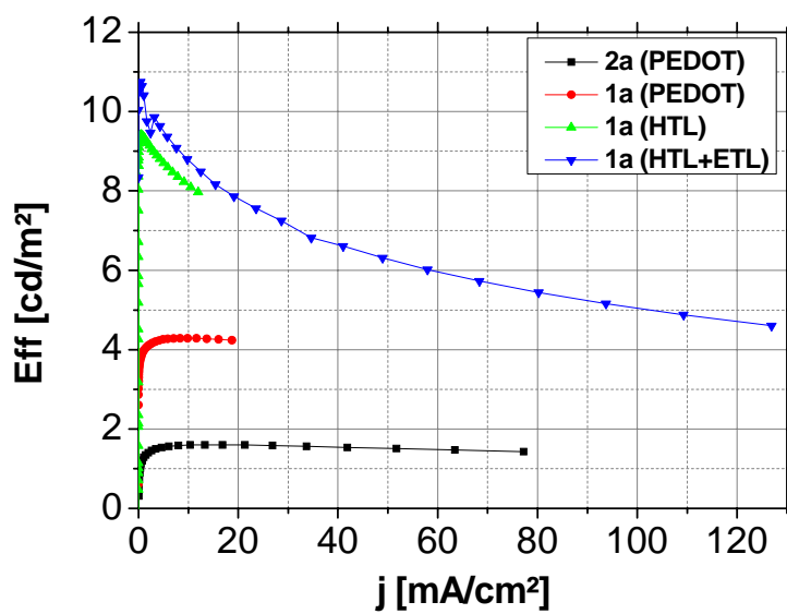
Fig S3 Typical efficiency versus current density curves for the screened devices.
