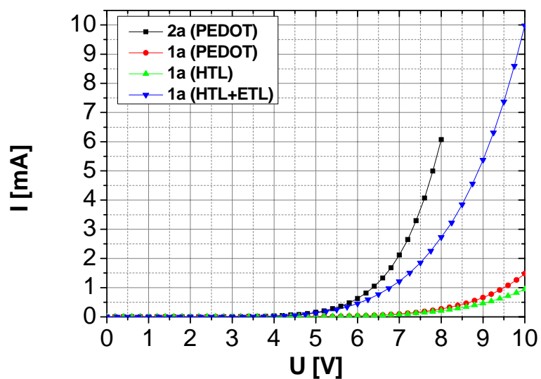
Fig S1 Typical current versus voltage curves for the screened devices.
