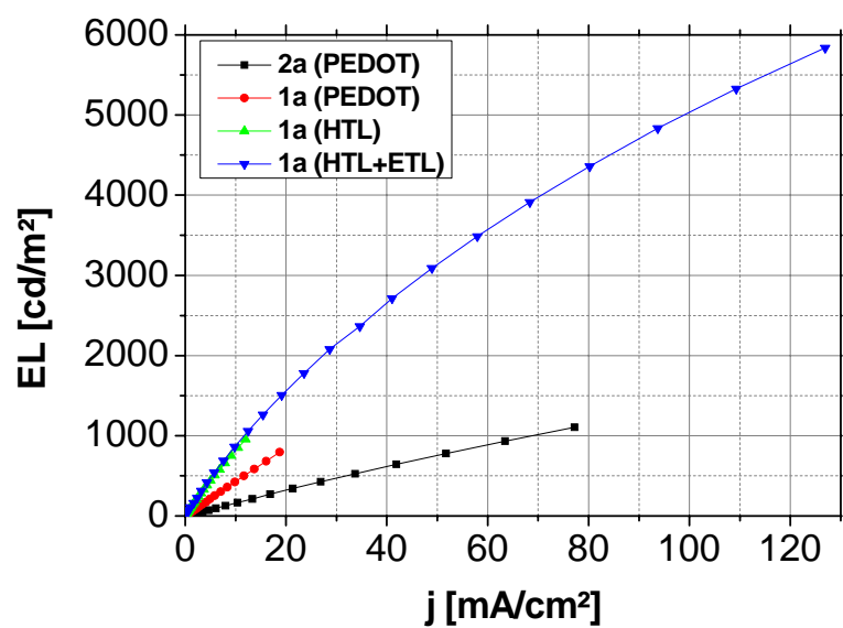
Fig S2 Typical brightness versus current density curves for the screened devices.
