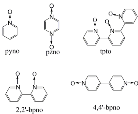
Fig. S1 The structures of pyridine N -oxide derivatives.
