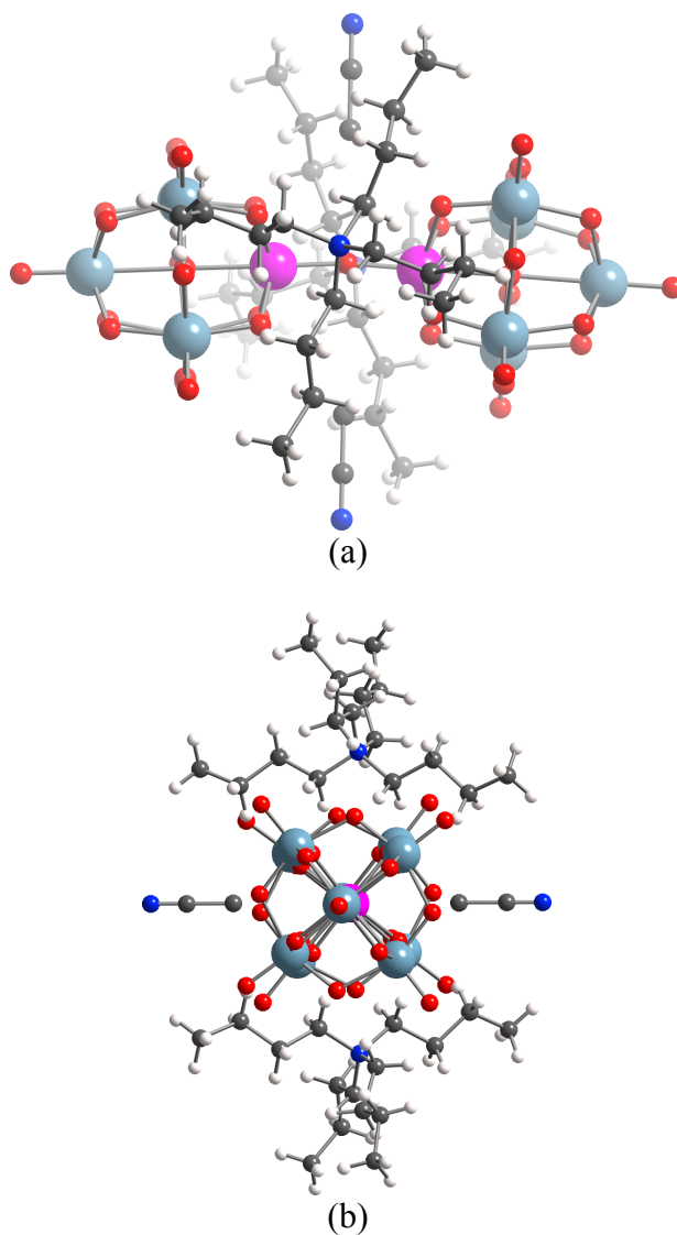
Figure S1 Views of anion 7 and adjacent TBA cations and MeCN molecules in the structure of (\text{TBA})_3[(\mu\text{-O})(\text{TiMo}_5\text{O}_{18})_2]2\text{MeCN}
