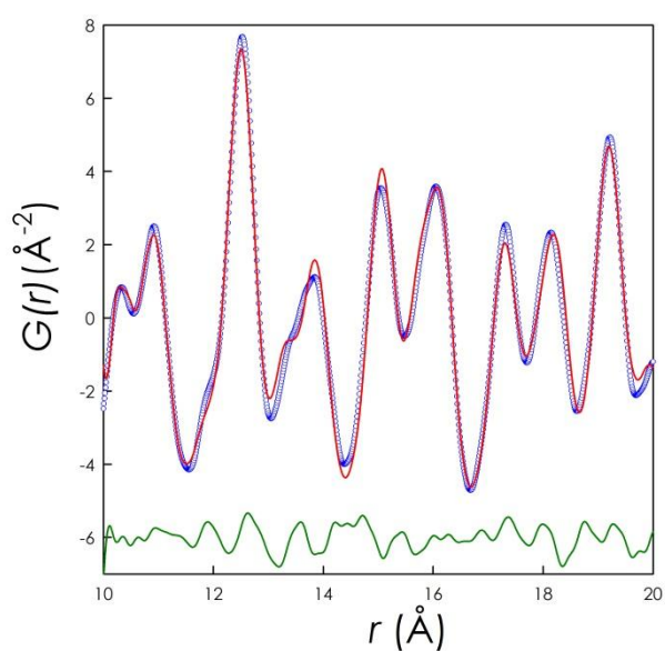
Fig. 1 PDF fit of \text{Ba}_2\text{In}_{1.7}\text{S}_{0.3}\text{O}_{5.45} from 10 to 20 Å with Pm\bar{3}m space group. Blue circles: experimental data; red line: calculated PDF; horizontal green line: residual.
