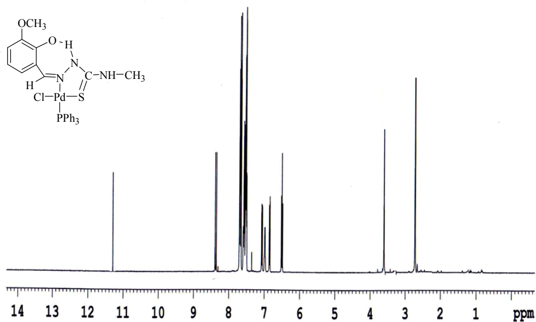
Fig. S4 1 H-NMR spectrum of [Pd(H-Msal-mtsc)(PPh 3 )](2)
