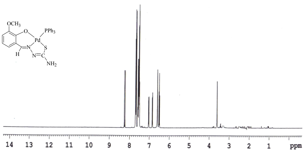
Fig. S2 ^1\text{H} -NMR spectrum of [\text{Pd}(\text{Msal-tsc})(\text{PPh}_3)](1)
