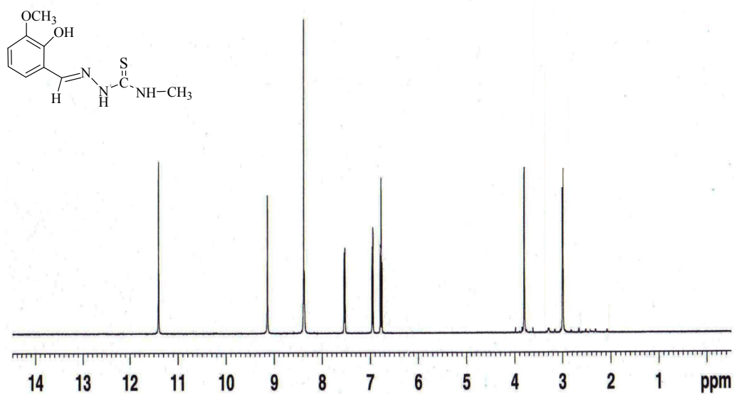
Fig. S3 1 H-NMR spectrum of (H 2 L 2 )
