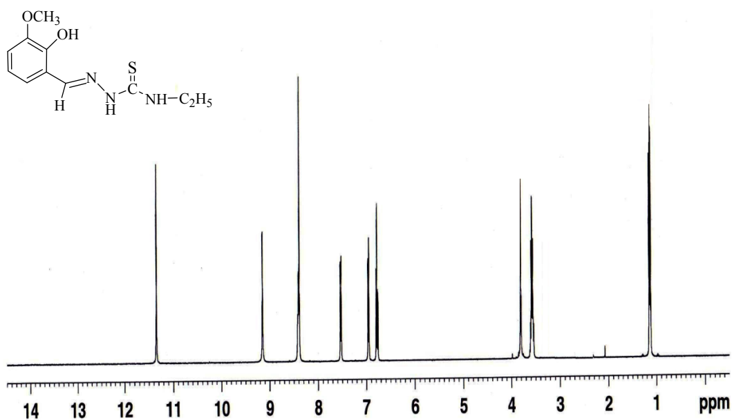
Fig. S5 1 H-NMR spectrum of (H 2 L 3 )
