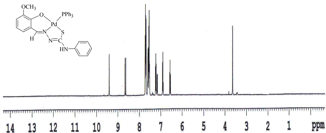
Fig. S8 ^1\text{H} -NMR spectrum of [\text{Pd}(\text{Msal-ptsc})(\text{PPh}_3)](4)
