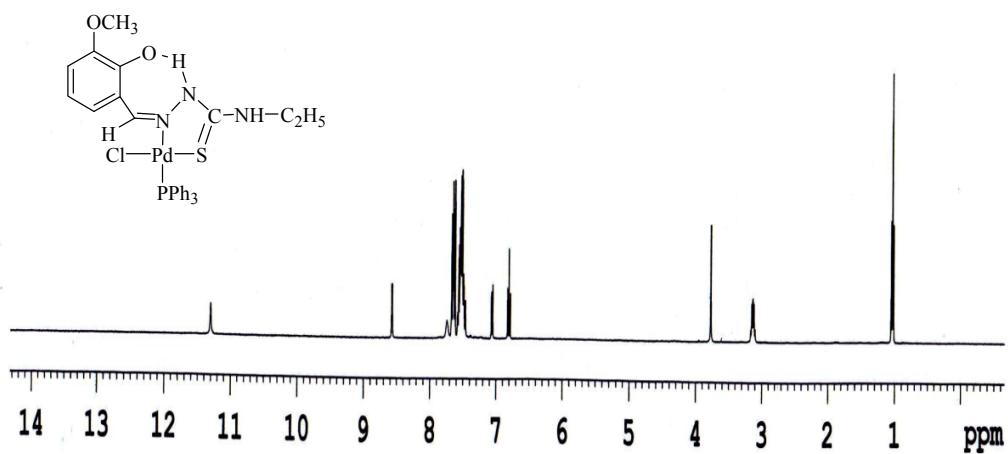
Fig.S6 1 H-NMR spectrum of [Pd(H-Msal-etsc)(PPh 3 )](3)
