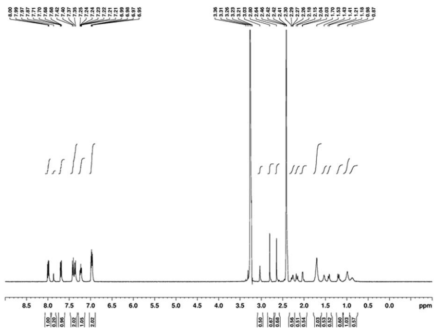
Fig. S1. ^1\text{H-NMR} spectrum of compound 3 in \text{DMSO-d}_6 .
