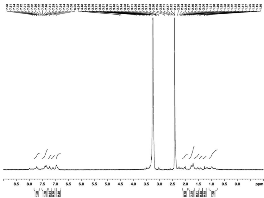
Fig. S2. ^1\text{H-NMR} spectrum of compound 6 in \text{DMSO-d}_6 .
