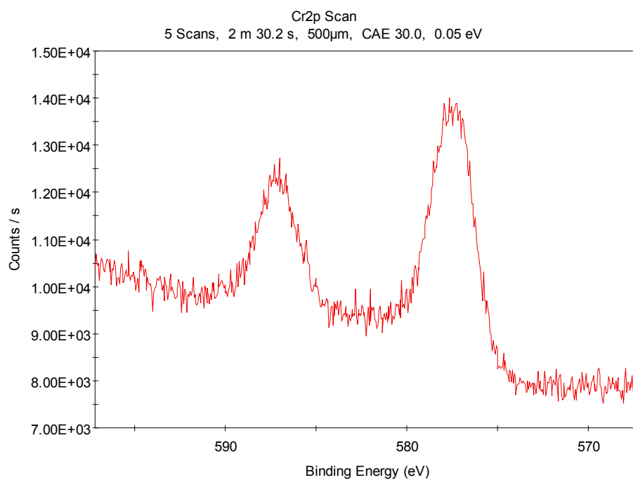
SFigure 1. The XPS spectrum of complex 4 .
