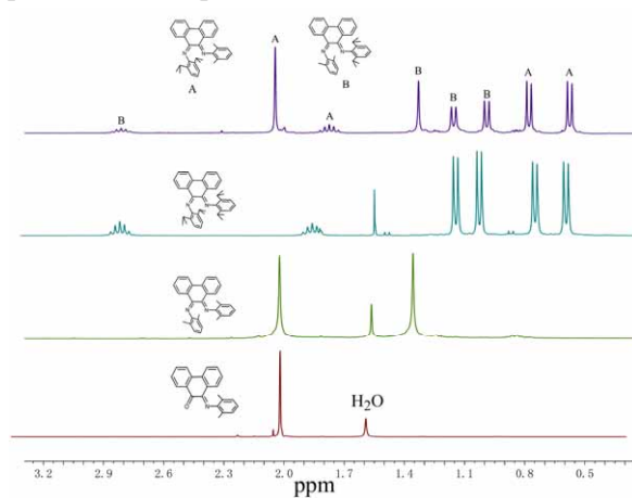
SFigure 2. Stacked 1 H NMR of L1 , L4 , L6 , and L7
