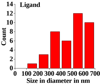
Figure S15: Particle size distribution of L from TEM analysis.
