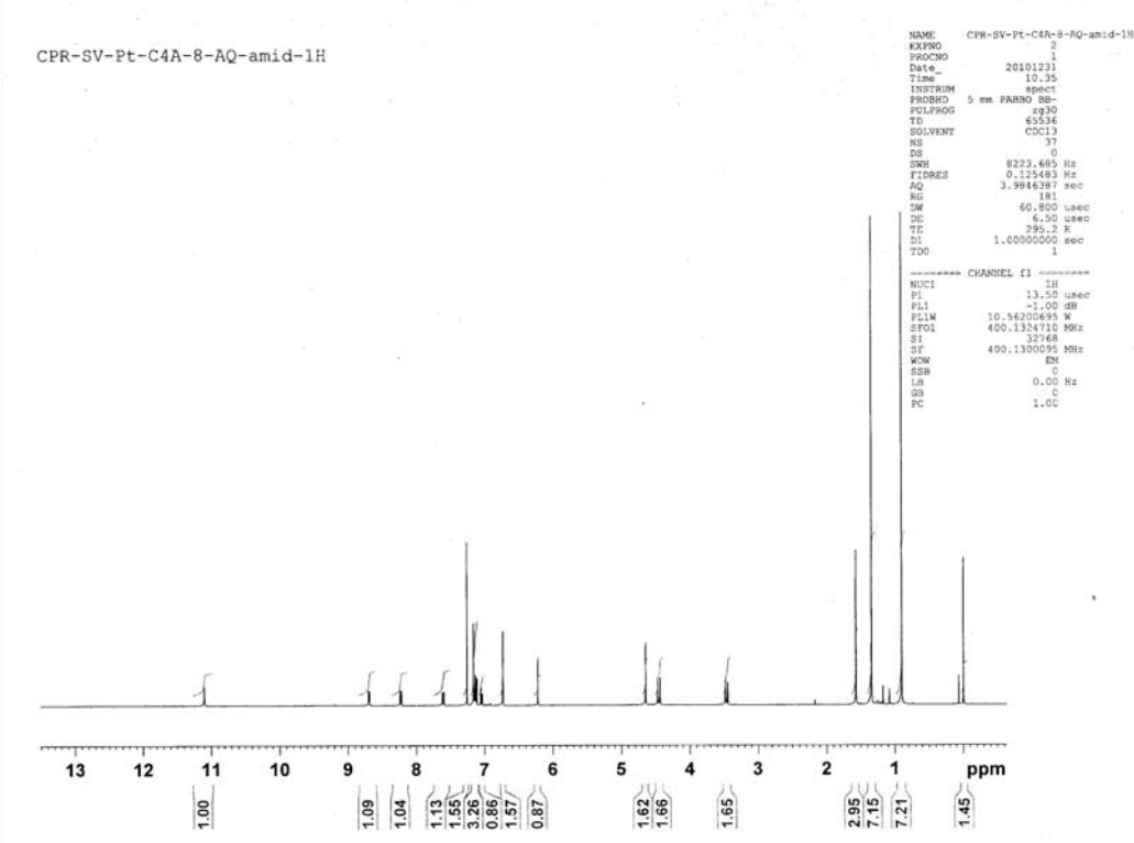
(a) ^1\text{H} -NMR spectrum of L
