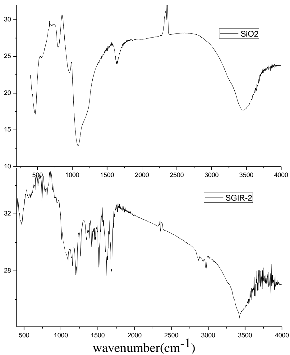
Figure S1. IR spectra of pure SiO 2 and SGIR-2 .
