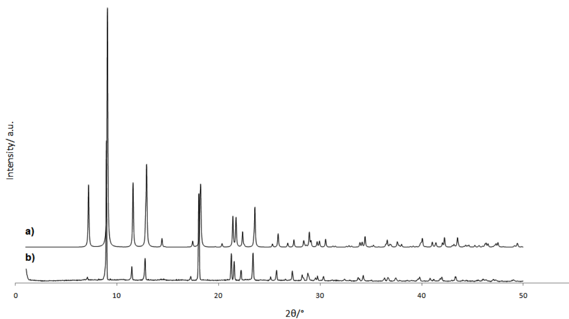
Fig. S1. a) PXRD pattern simulated from single crystal structural data for 1 ; b) experimental PXRD pattern of 1 .
