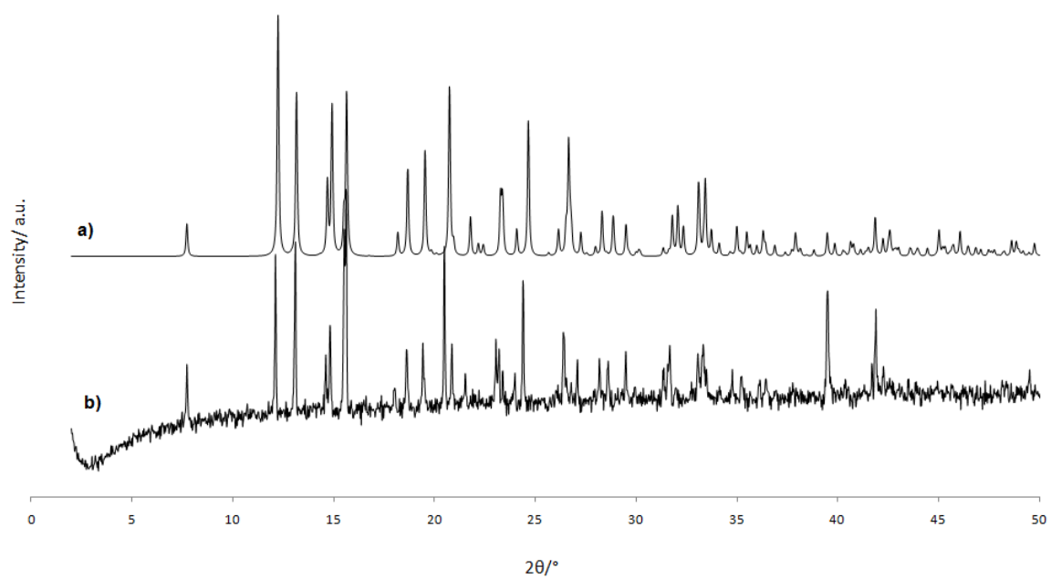
Fig. S2. a) PXRD pattern simulated from single crystal structural data for 2 b) experimental PXRD pattern of 2 .
