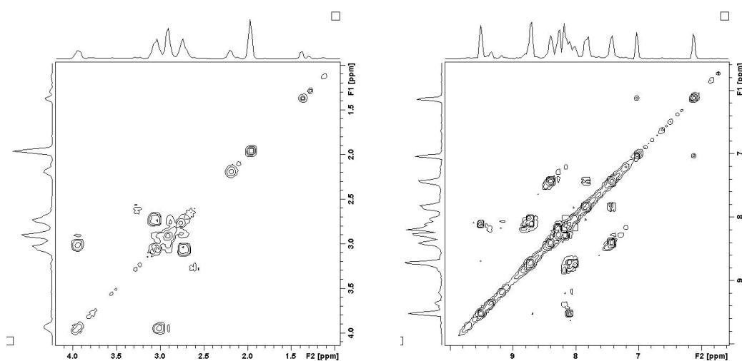
Figure S1: ( ^1\text{H} - ^1\text{H} )COSY spectra for complex 2A in \text{CD}_3\text{CN} .
