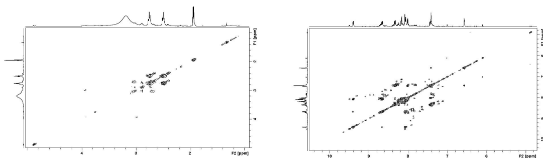
Figure S3: ( ^1\text{H} - ^1\text{H} )COSY spectra for complex ( 1R+2A ) in \text{CD}_3\text{CN} .
