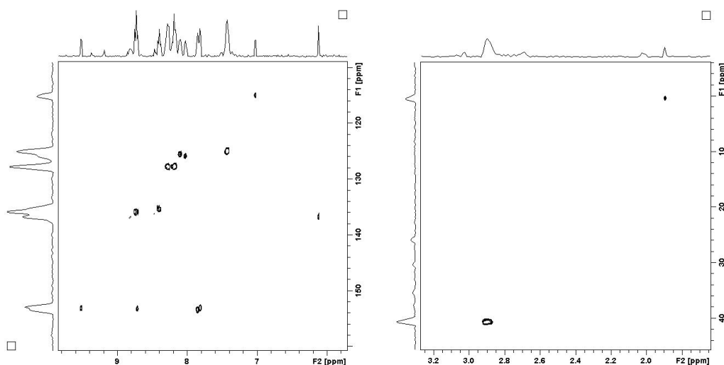
Figure S2: ( ^1\text{H} - ^{13}\text{C} )HSQC spectra for complex 2A in \text{CD}_3\text{CN} .
