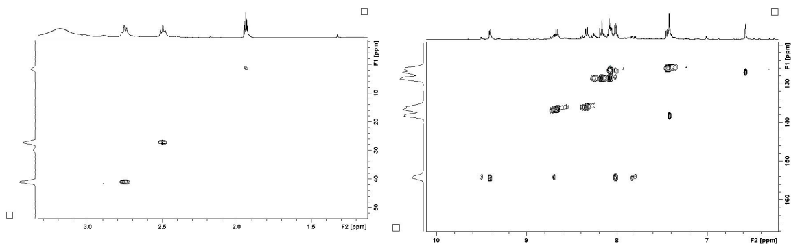
Figure S4: ( ^1\text{H} - ^{13}\text{C} )HSQC spectra for complex ( 1R+2A ) in \text{CD}_3\text{CN} .
