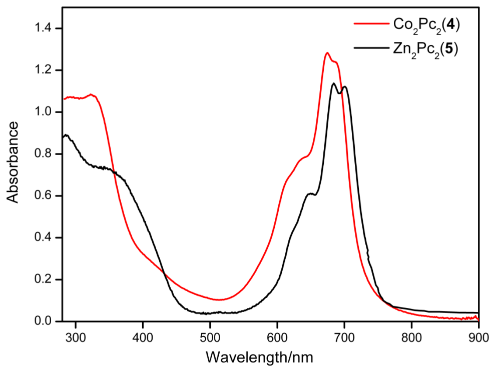
Fig. S1. Absorption spectra of 5.0 \times 10^{-5} M compound 4 and 5 in DMSO
