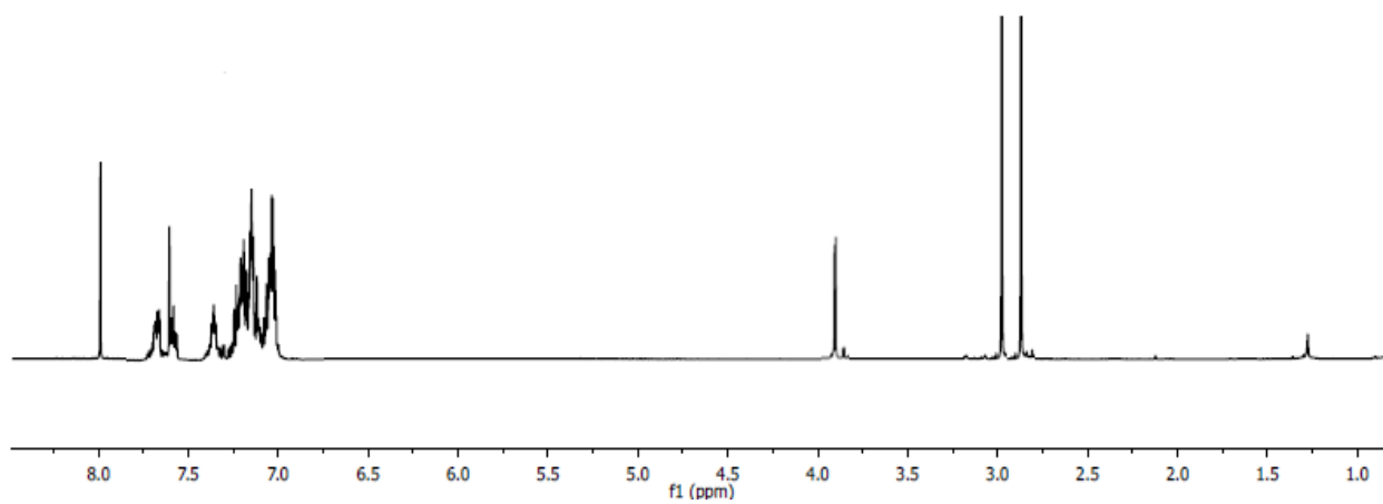
Fig. S2. 1 H-NMR spectrum of compound 5 in DMF.
