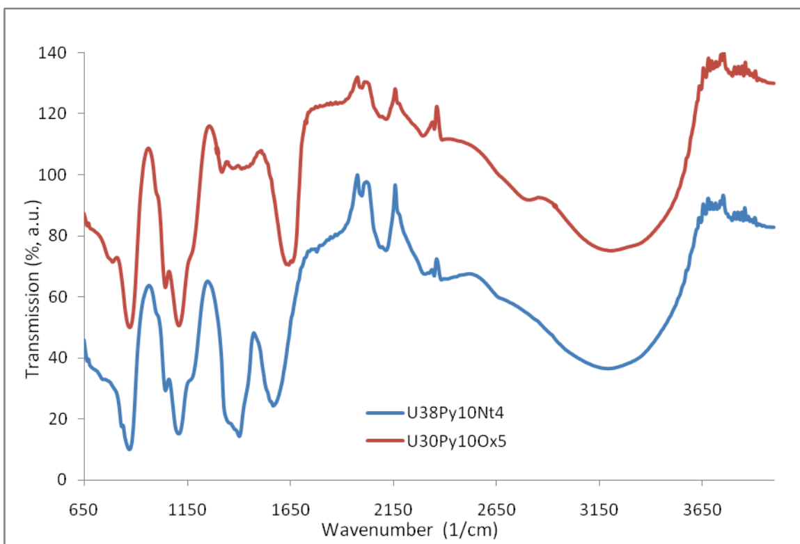
Figure S1. Infrared spectra of U_{30}Py_{10}Ox_5 (red) and U_{38}Py_{10}Nt_4 (blue).
