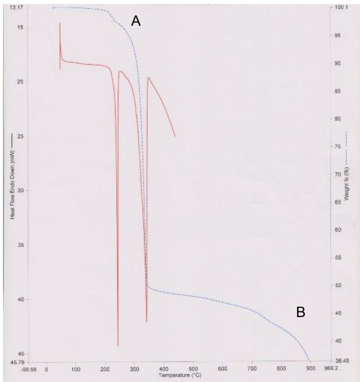
DSC and TGA thermogram of \text{Pb}(\text{pip-dtc})_2
