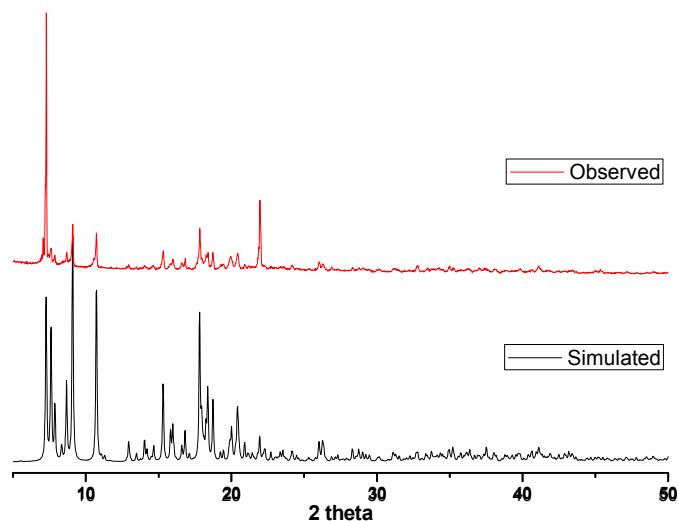
Figure S2. The observed and simulated X-ray diffraction patterns of complex α -5 .
