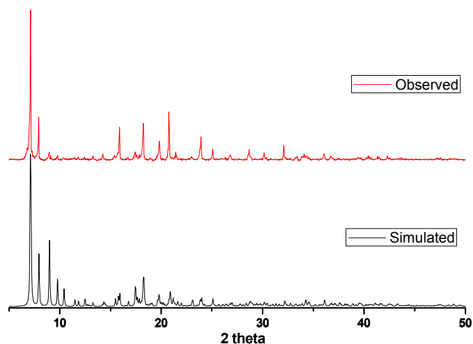
Figure S2. The observed and simulated X-ray diffraction patterns of complex α -5 .
